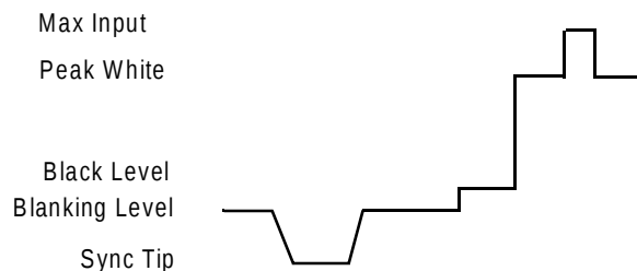
Figure 12. Luminance Signal
