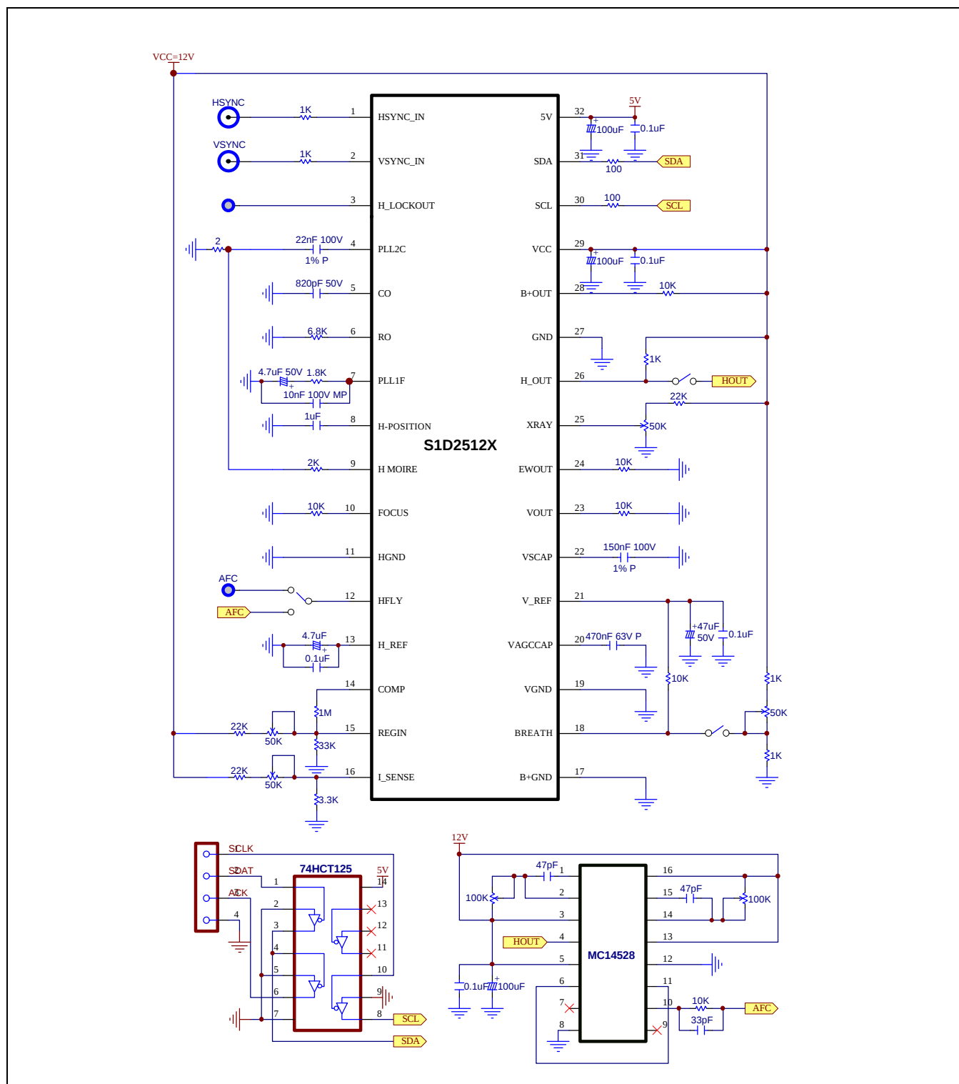
Figure 15. Application Circuit
