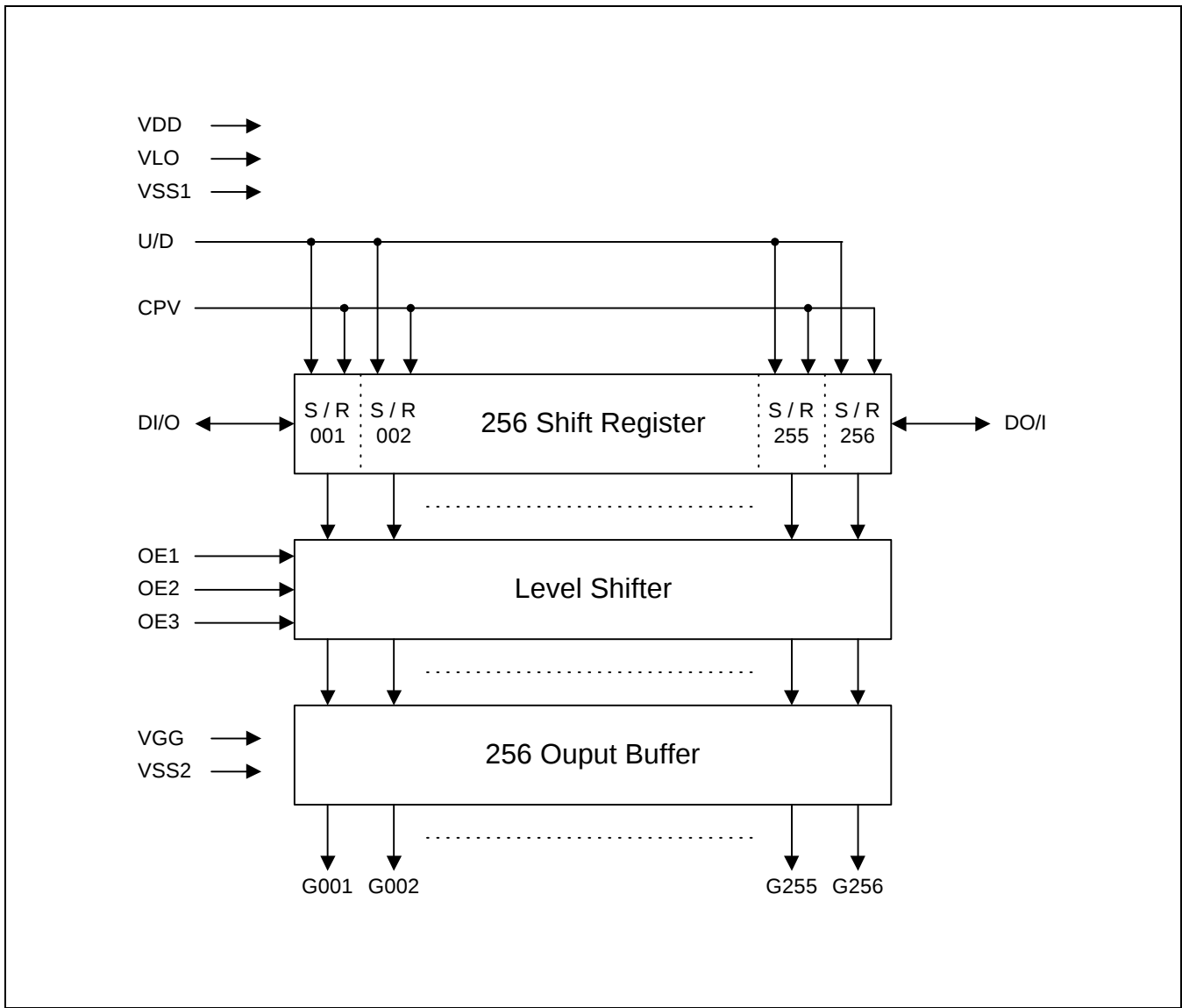
Figure 1. Block Diagram
