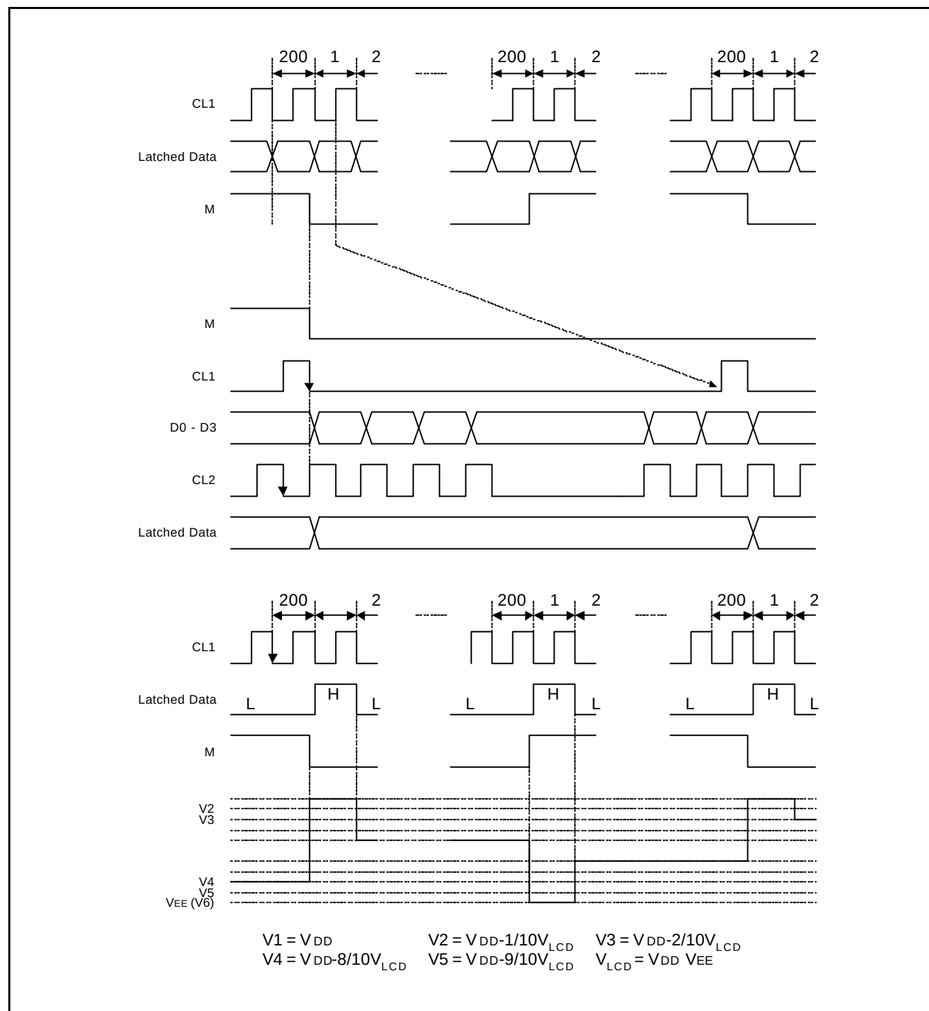
Timing Chart - 1/200 Duty, 1/15 Bias
