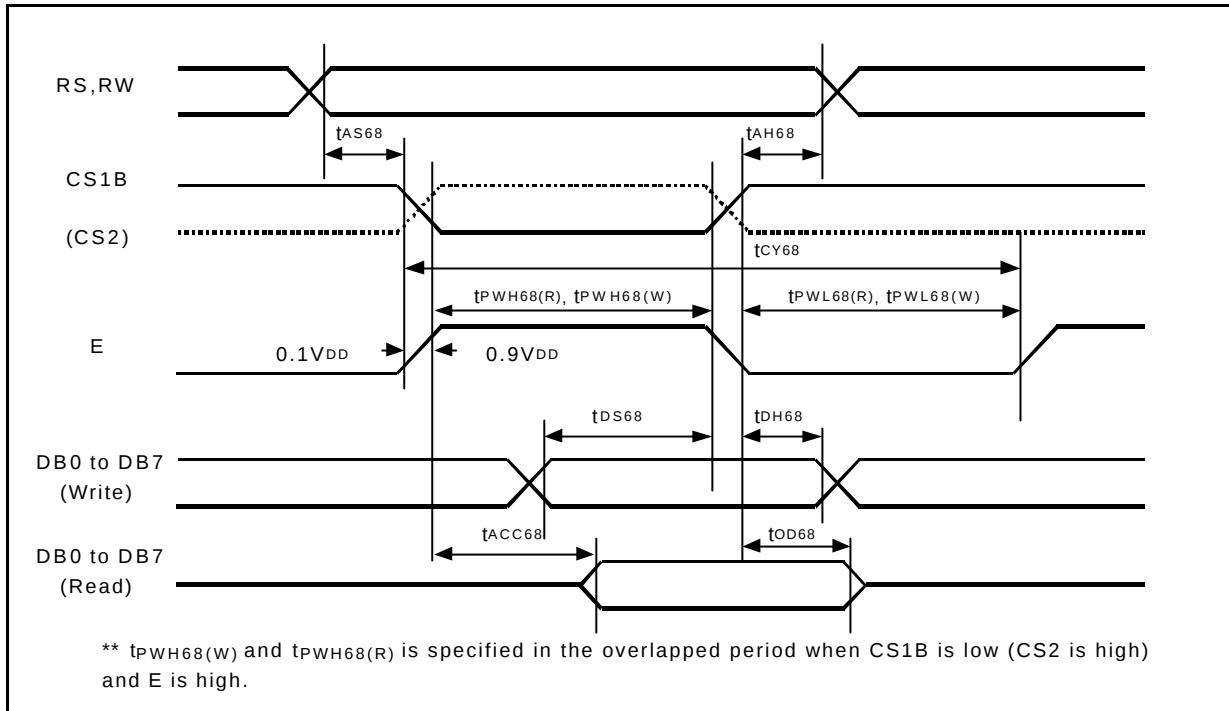
Figure 33. Read / Write Characteristics (6800-series Microprocessor)
