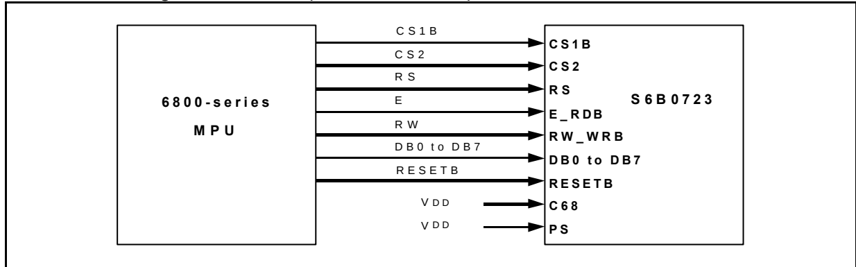
Figure 37. Interfacing with 6800-series (PS = "H", C68 = "H")
