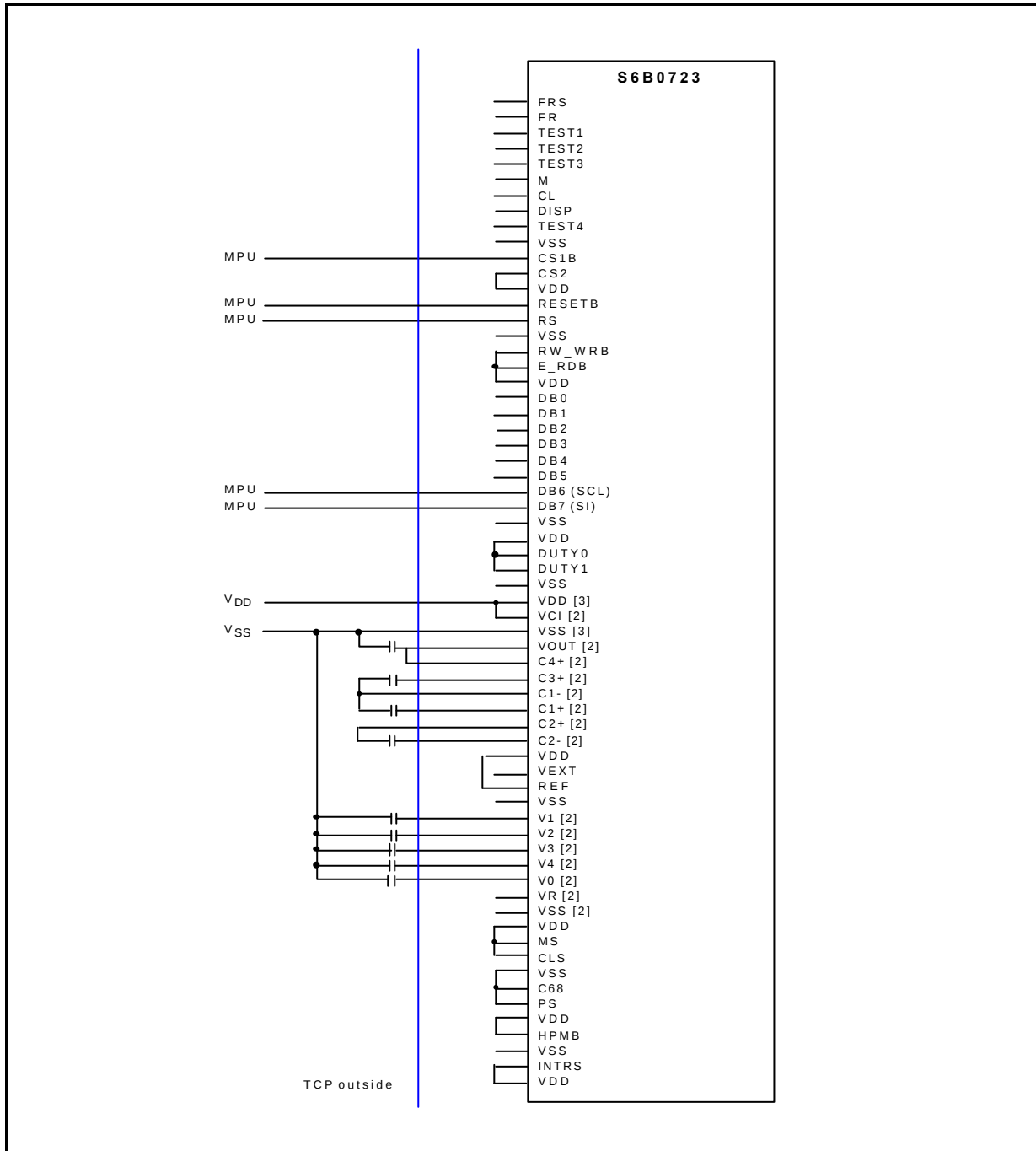
Figure 58. S6B0723 Application Circuit for Serial
