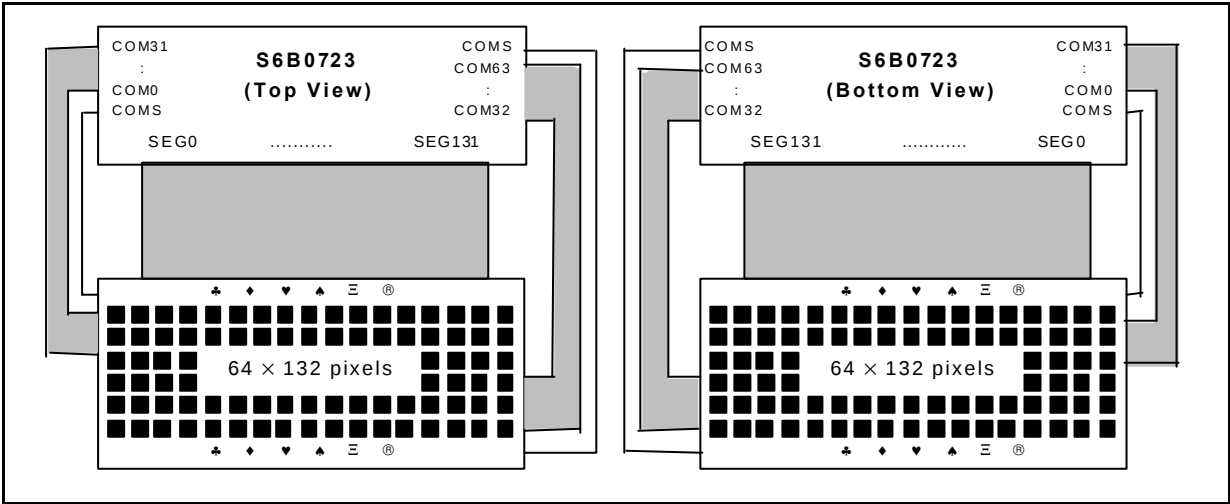
Figure 42. SHL = 0, ADC = 0
