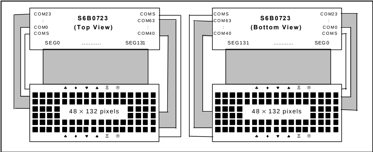
Figure 50. SHL = 0, ADC = 0
