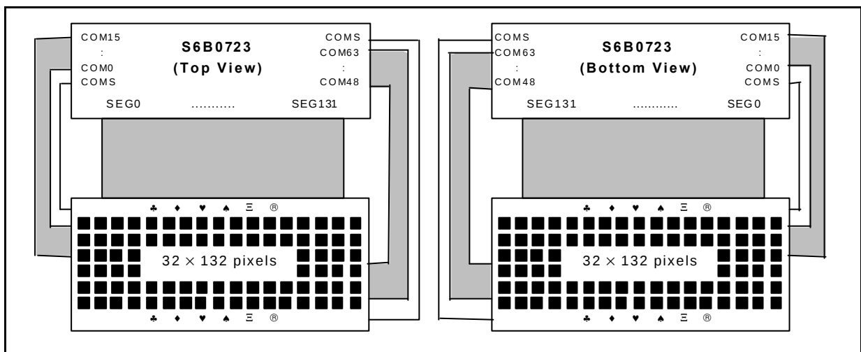
Figure 54. SHL = 0, ADC = 0
