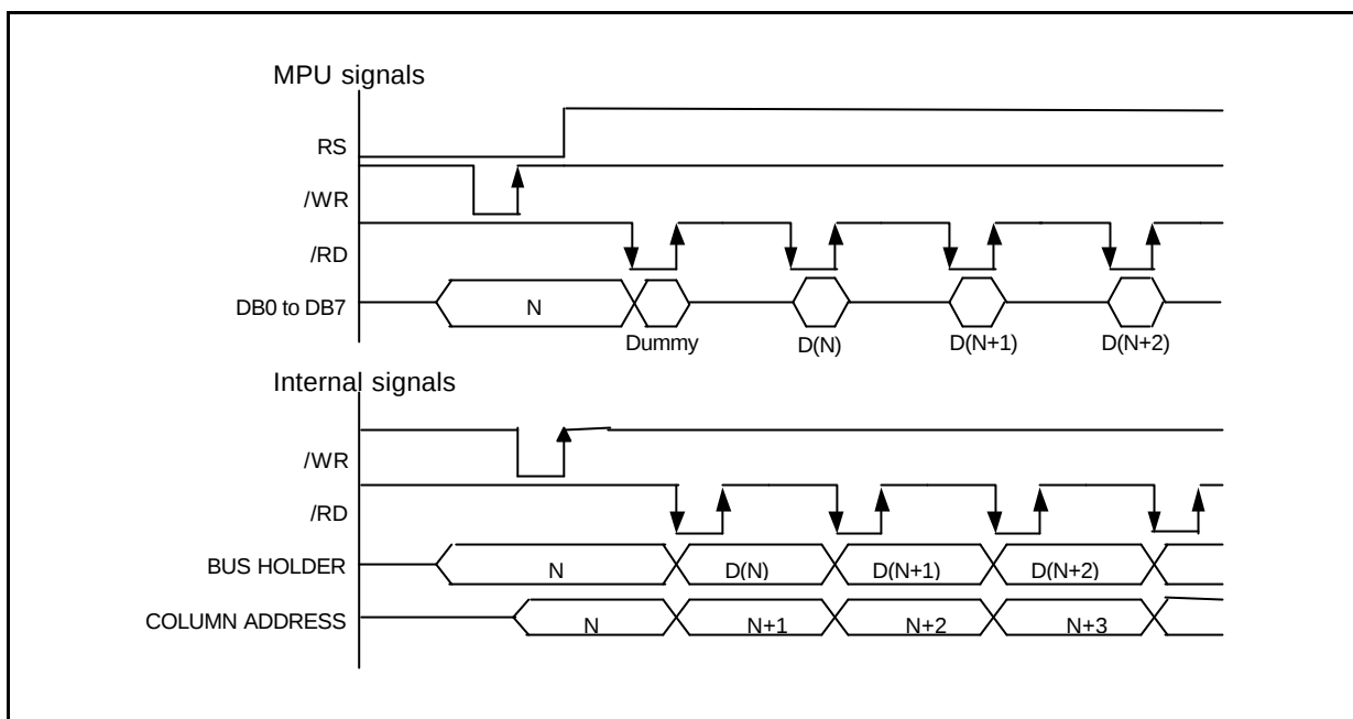
Figure 7. Read Timing
