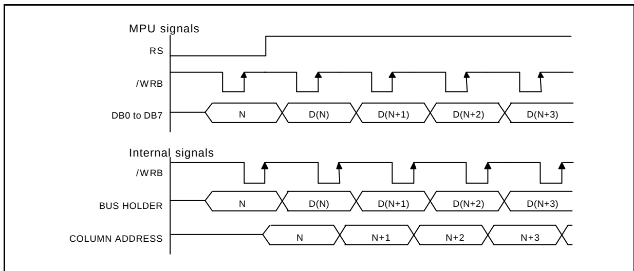
Figure 6. Write Timing
