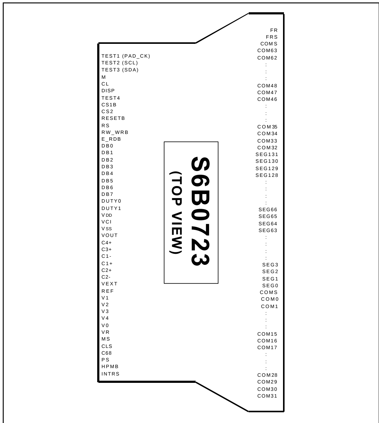
Figure 59. TCP Pin Layout
