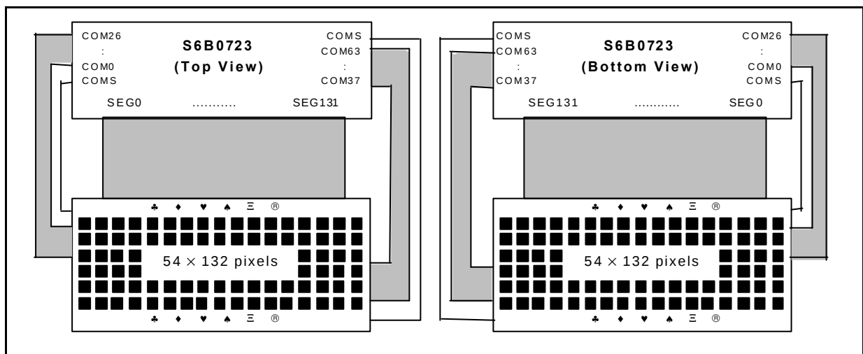
Figure 46. SHL = 0, ADC = 0
