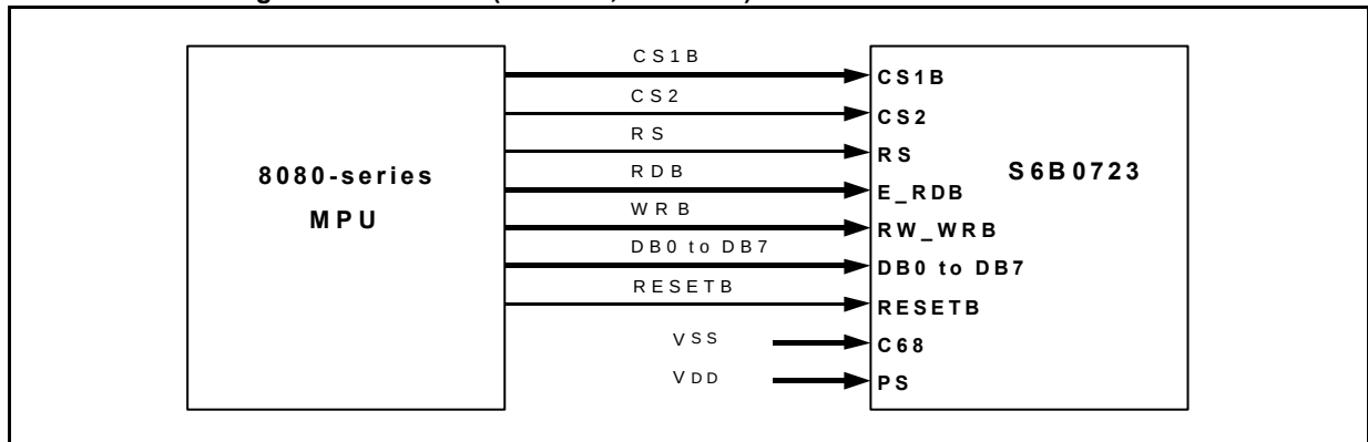
Figure 38. Interfacing with 8080-series (PS = "H", C68 = "L")
