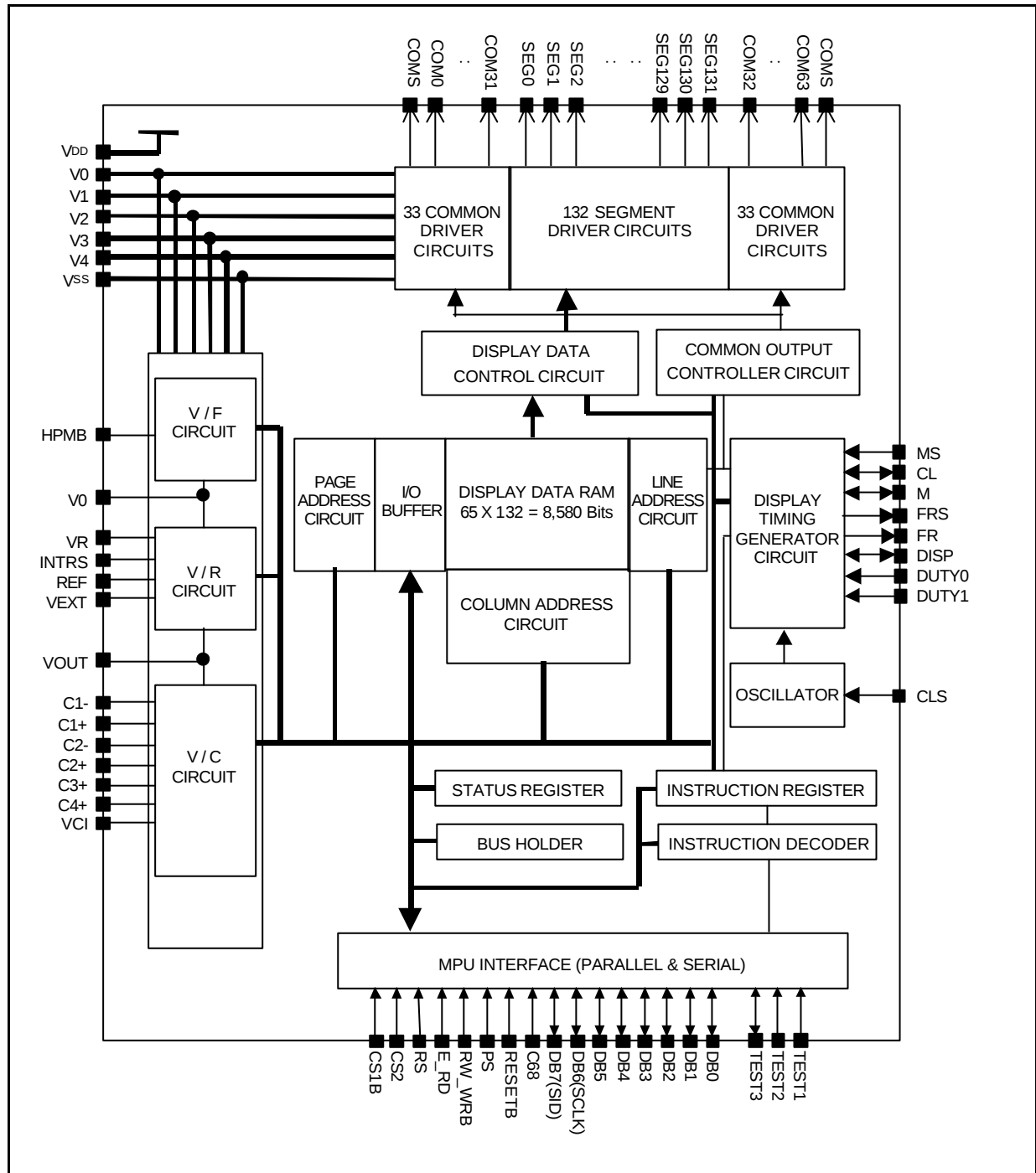
Figure 1. Block Diagram
