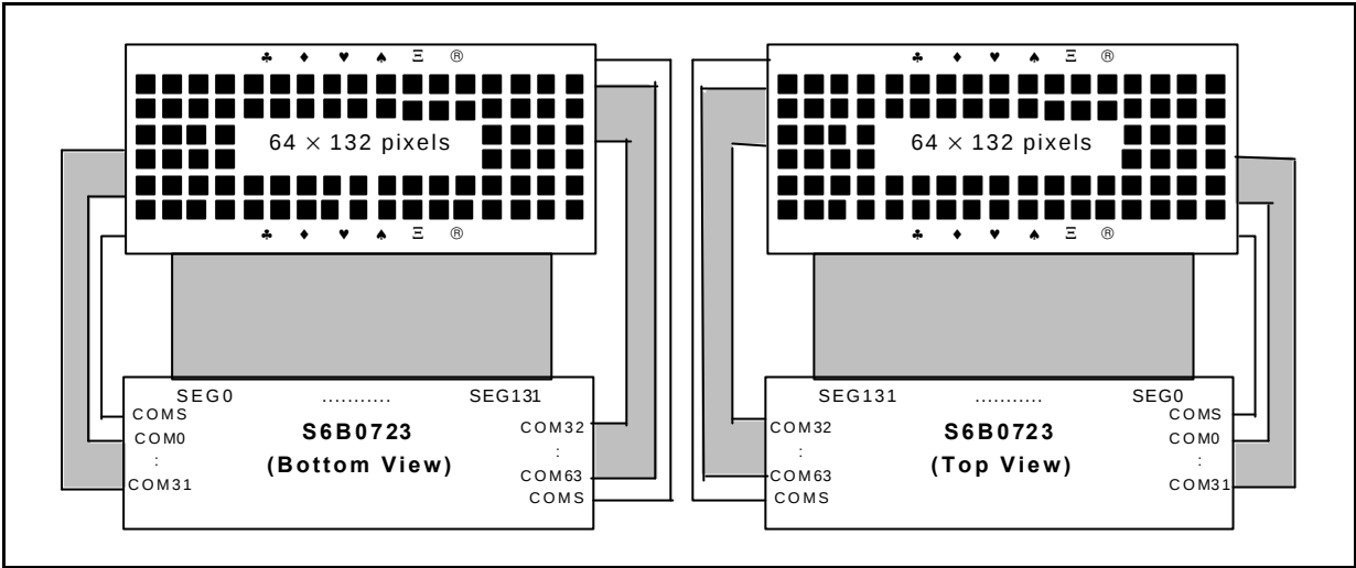
Figure 40. SHL = 1, ADC = 0
