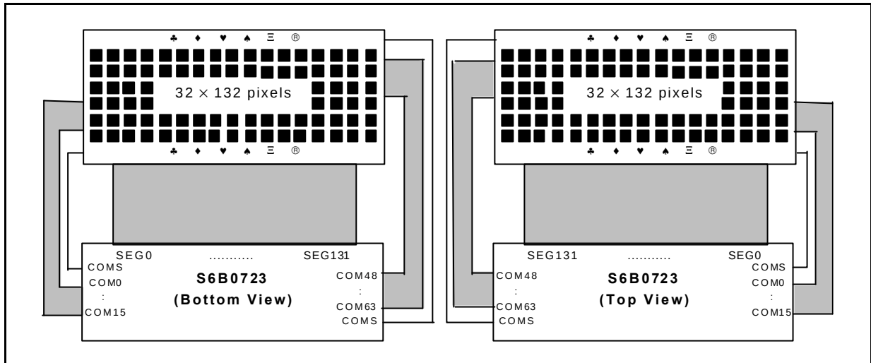
Figure 52. SHL = 1, ADC = 0
