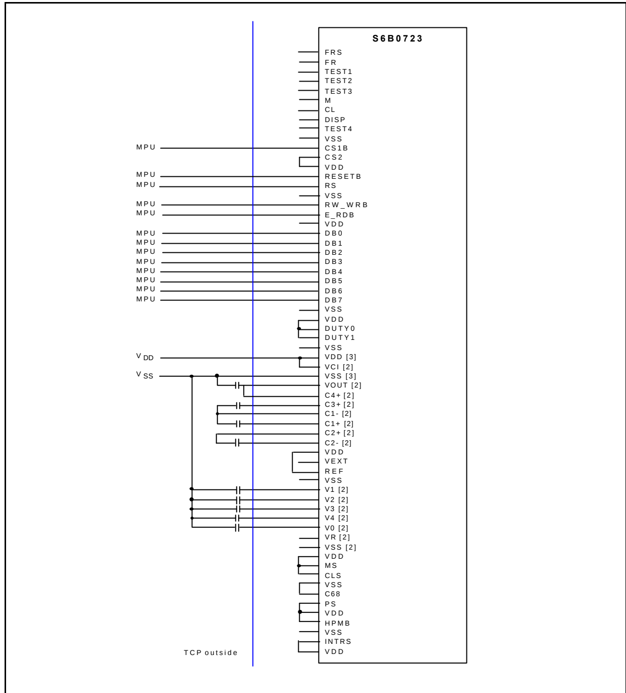
Figure 57. S6B0723 Application Circuit for 80-series
