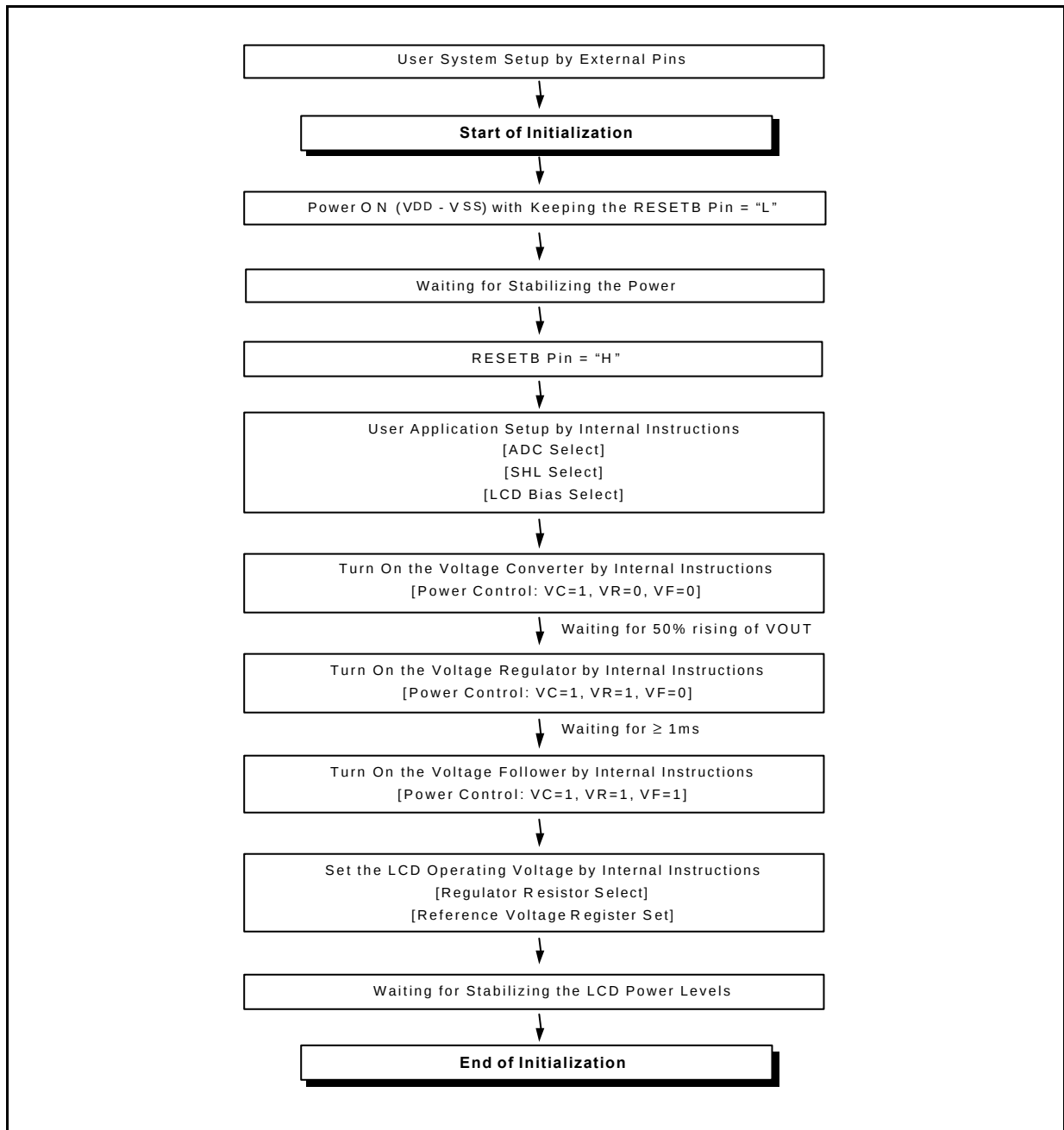
Figure 28. Initializing with the Built-in Power Supply Circuits
