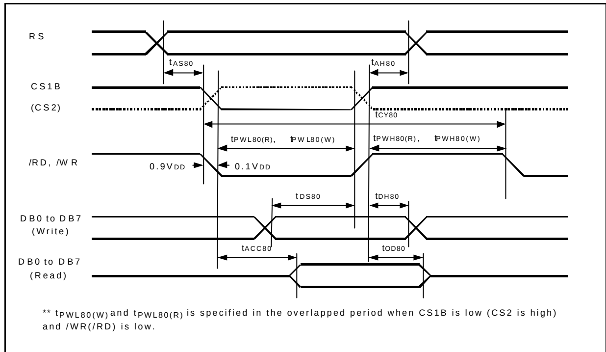
Figure 32. Read / Write Characteristics (8080-series MPU)
