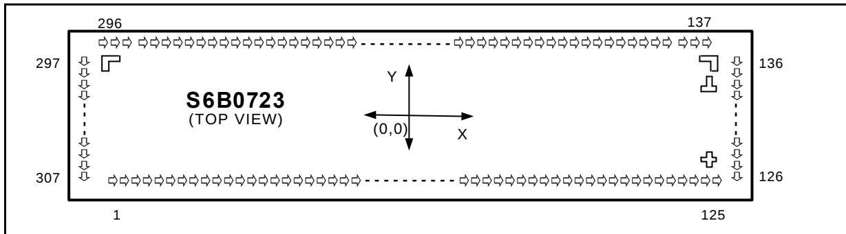
Figure 2. S6B0723 Chip Configuration
