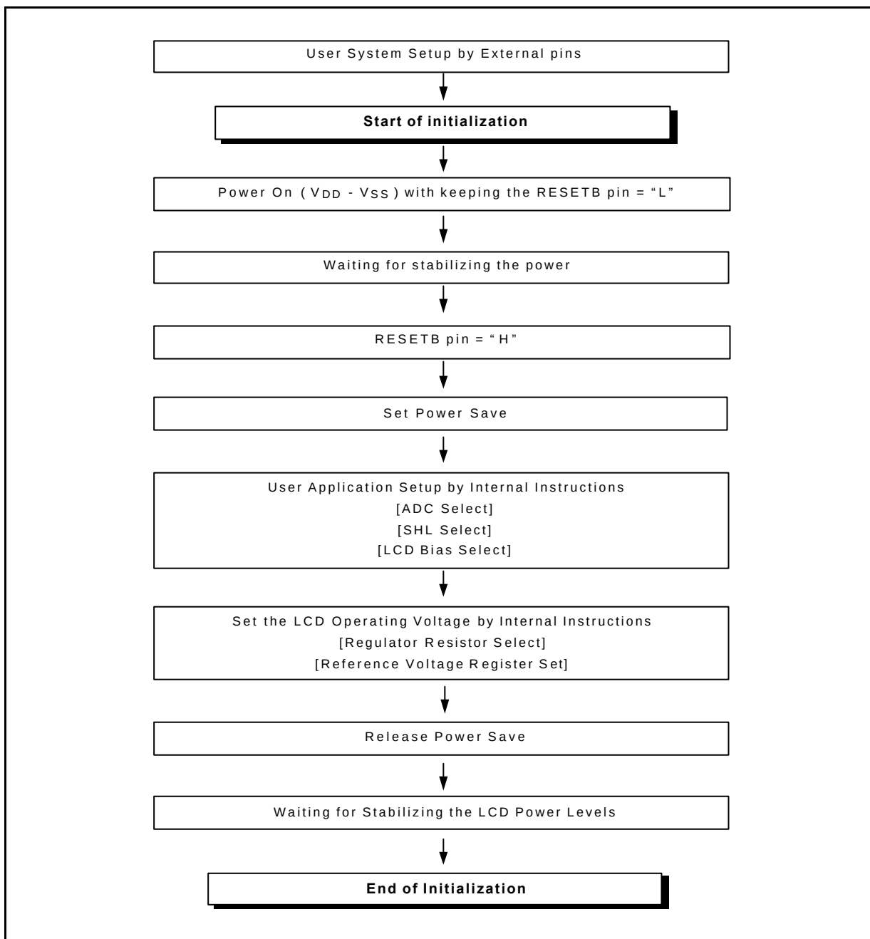
Figure 29. Initializing without the Built-in Power Supply Circuits
