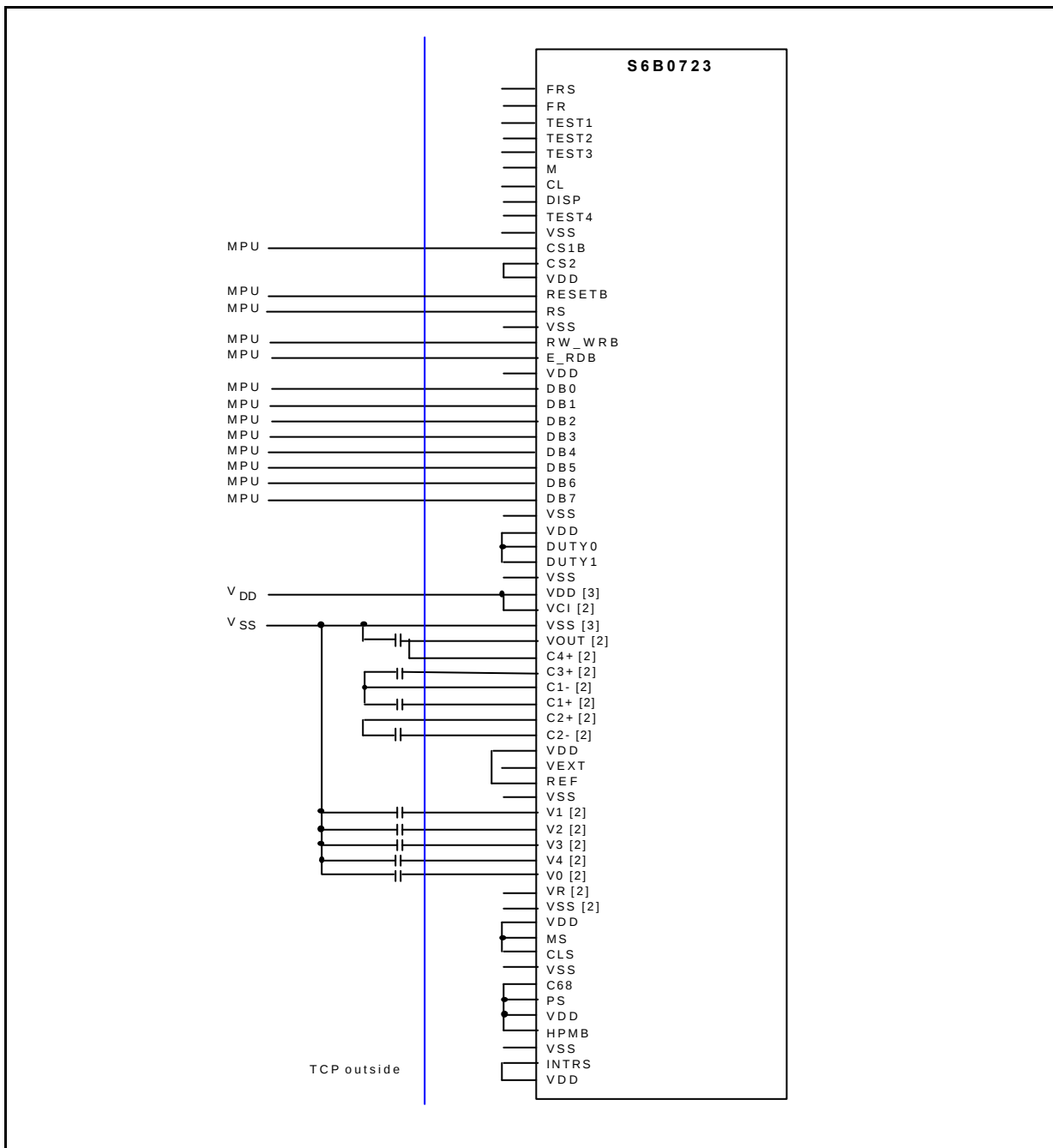
Figure 56. S6B0723 Application Circuit for 68-series
