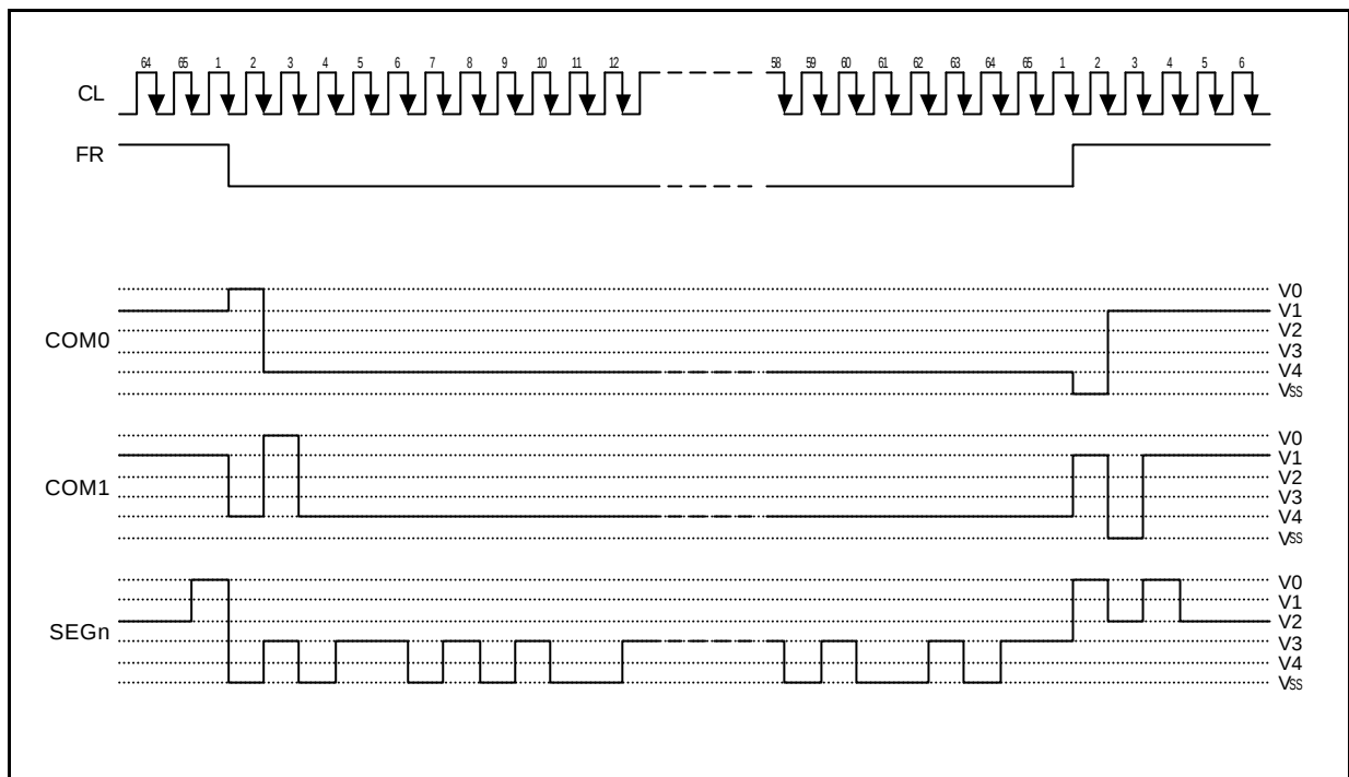
Figure 11. 2-frame AC Driving Waveform (Duty Ratio = 1/65)
