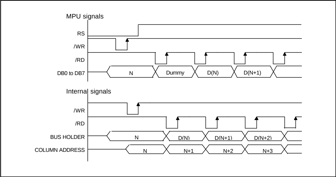
Figure 7. Read Timing
