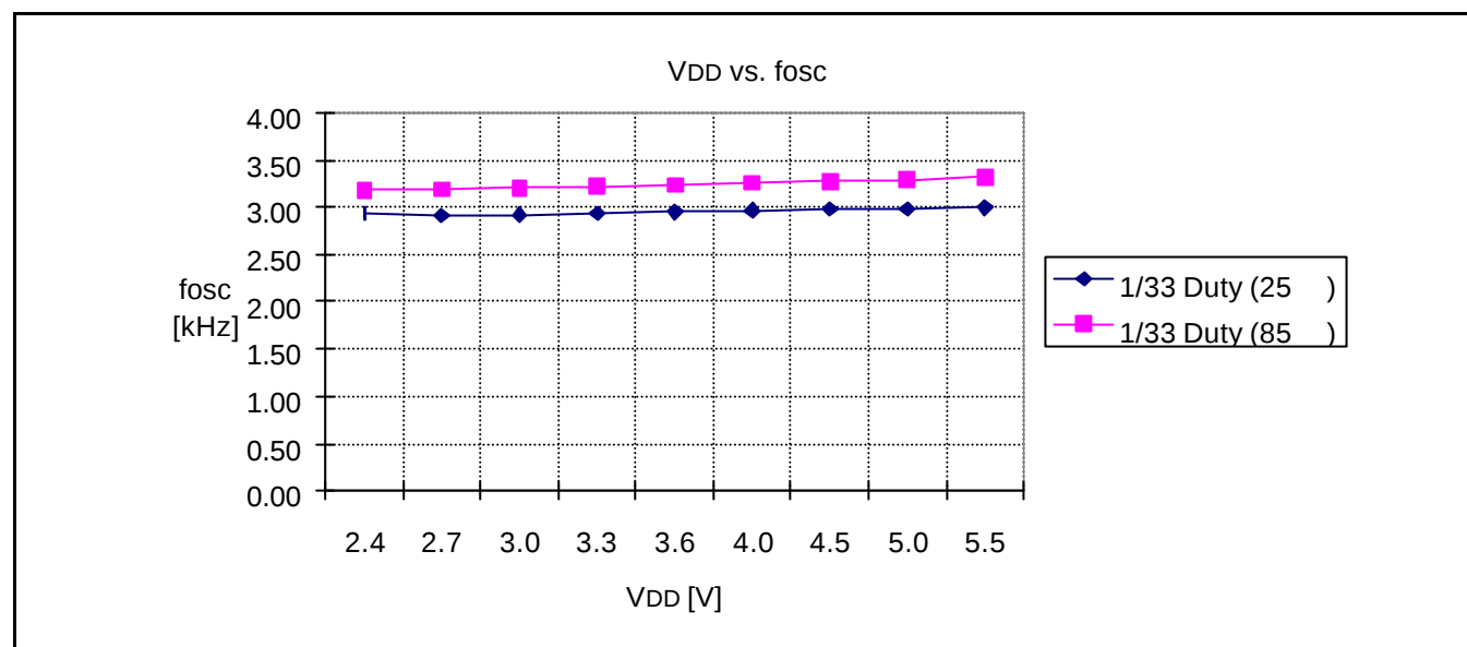
Figure 11. VDD vs. fosc
