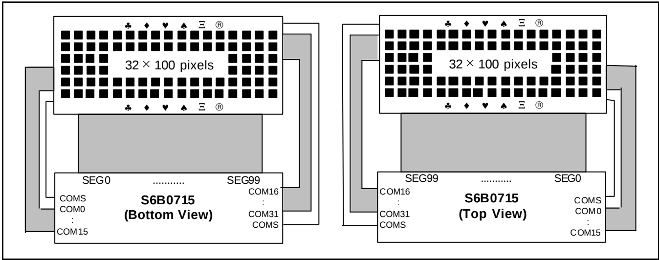
Figure 44. SHL = 1, ADC = 0
