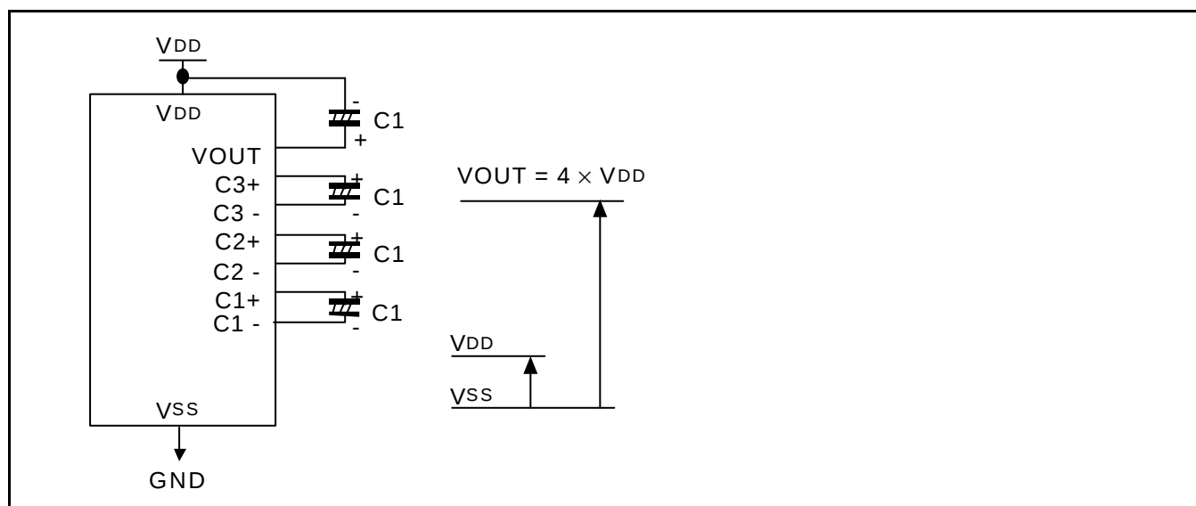
Figure 16. Four Times Boosting Circuit
