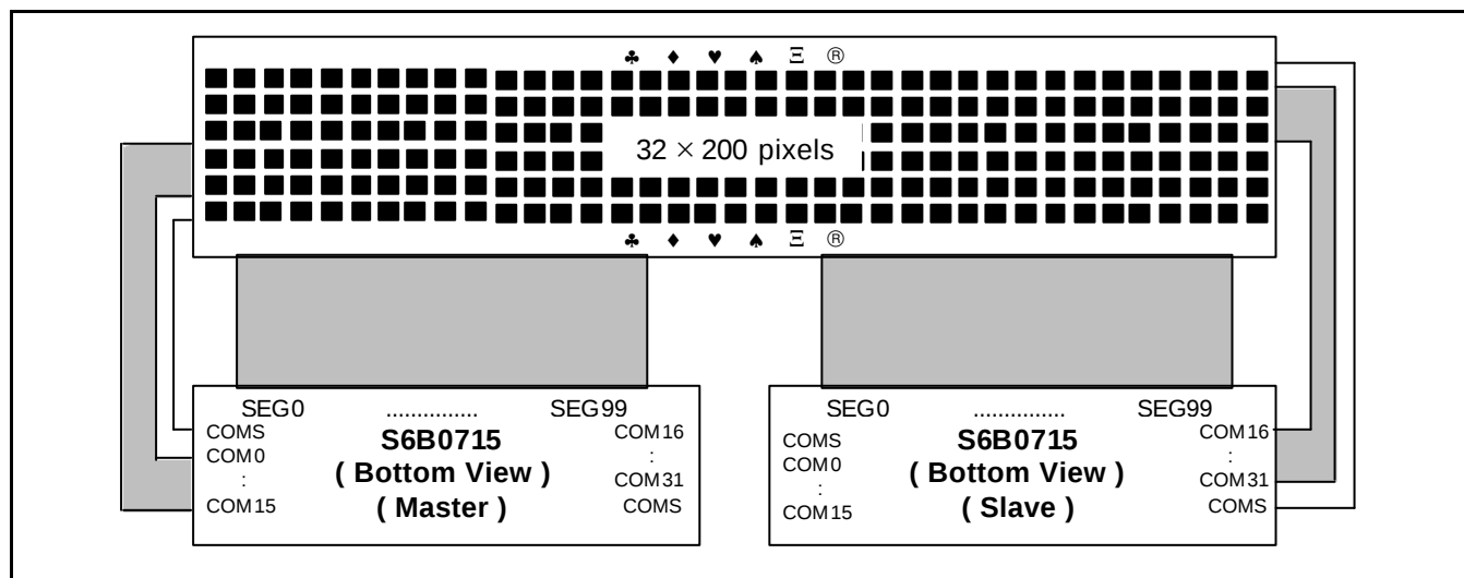
Figure 47. SHL = 1, ADC = 0
