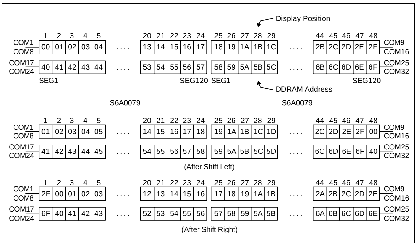
Figure 2. 2-line X 48ch. Display (5-dot Font Width)
