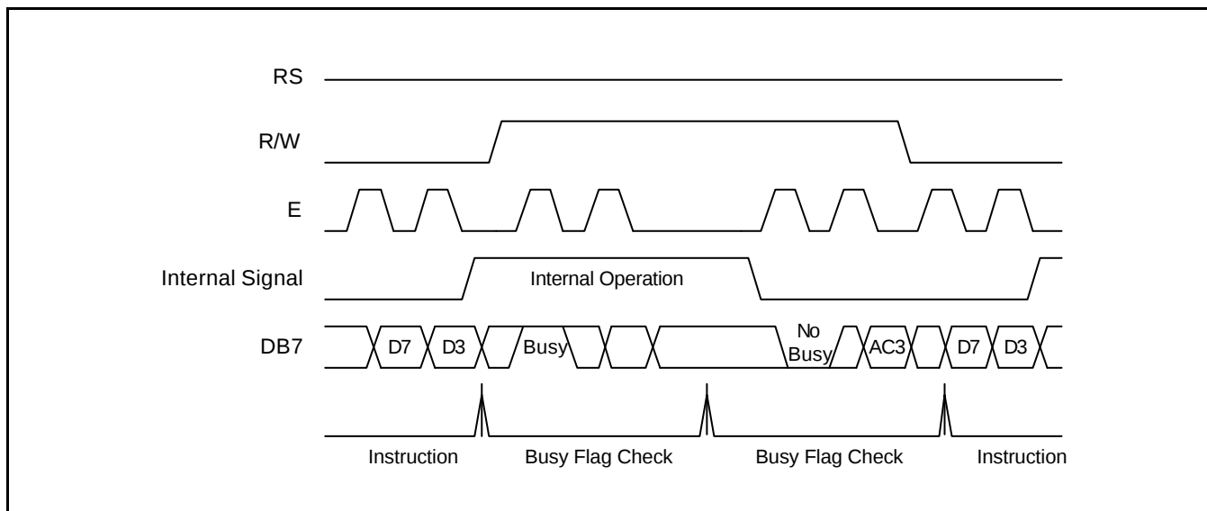
Figure 6. Example of 4-bit Bus Mode Timing Sequence
