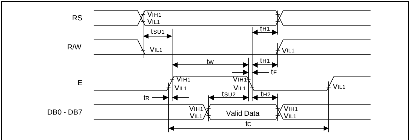
Figure 7. Write Mode
