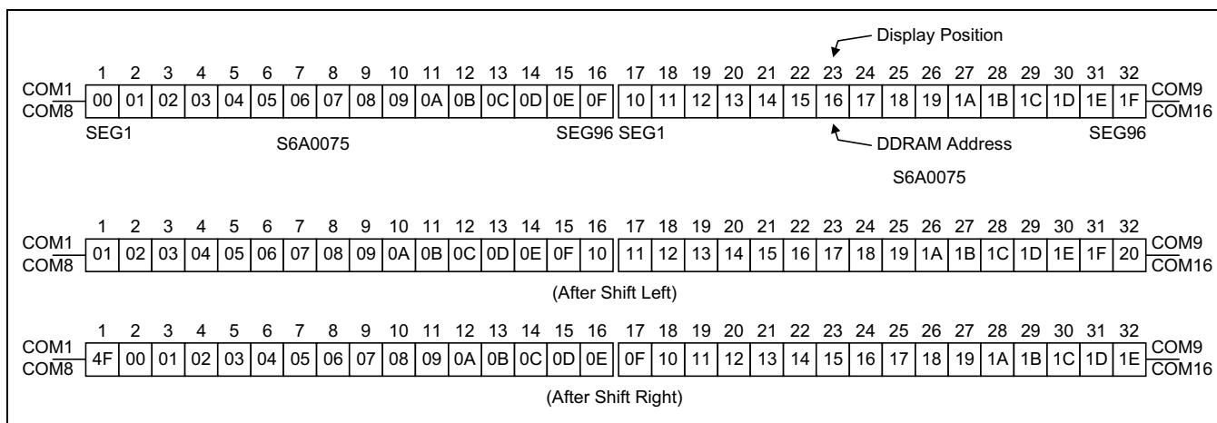
Figure 5. 1-line × 32ch. Display
