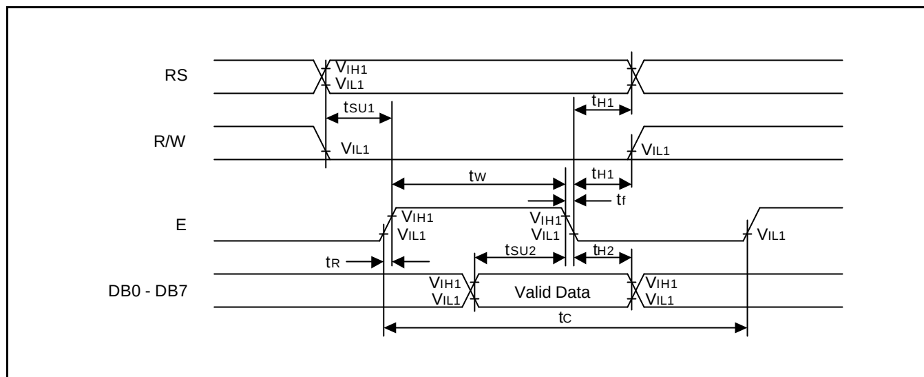
Figure 6. Write Mode Timing Diagram
