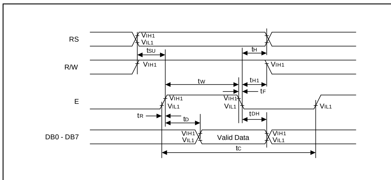
Figure 7. Read Mode Timing Diagram
