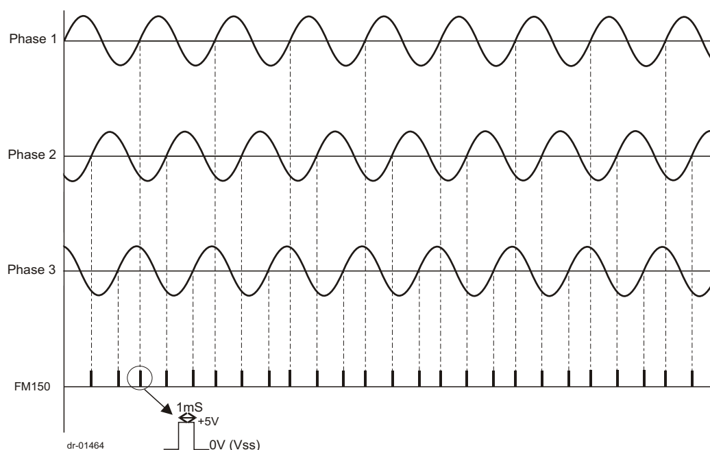
Figure 4: Mains voltage zero corssover pin FMO
