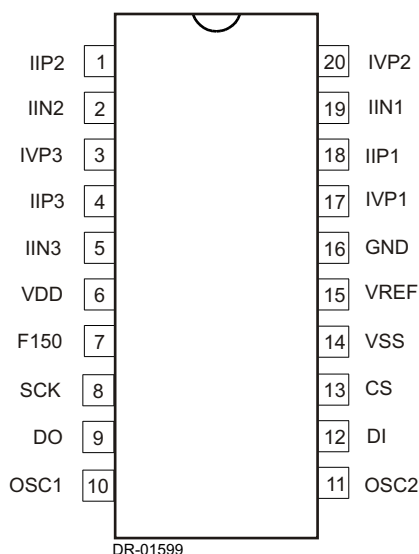
Figure 2: Pin connections: Package: DIP-20, SOIC-20
