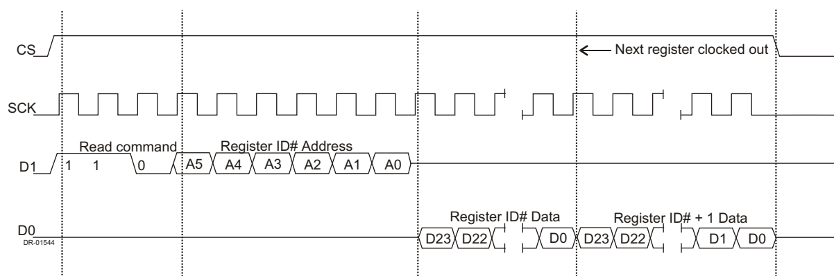
Figure 5: SPI waveforms
