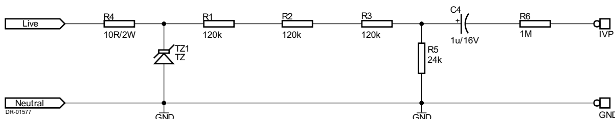
Figure 4: Mains voltage divider
