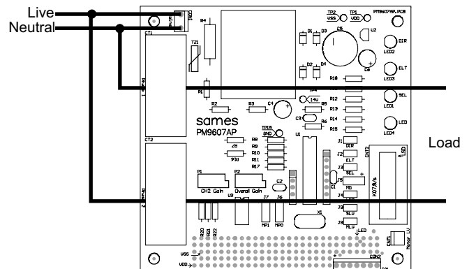
Figure 1: Connection diagram for normal metering application
