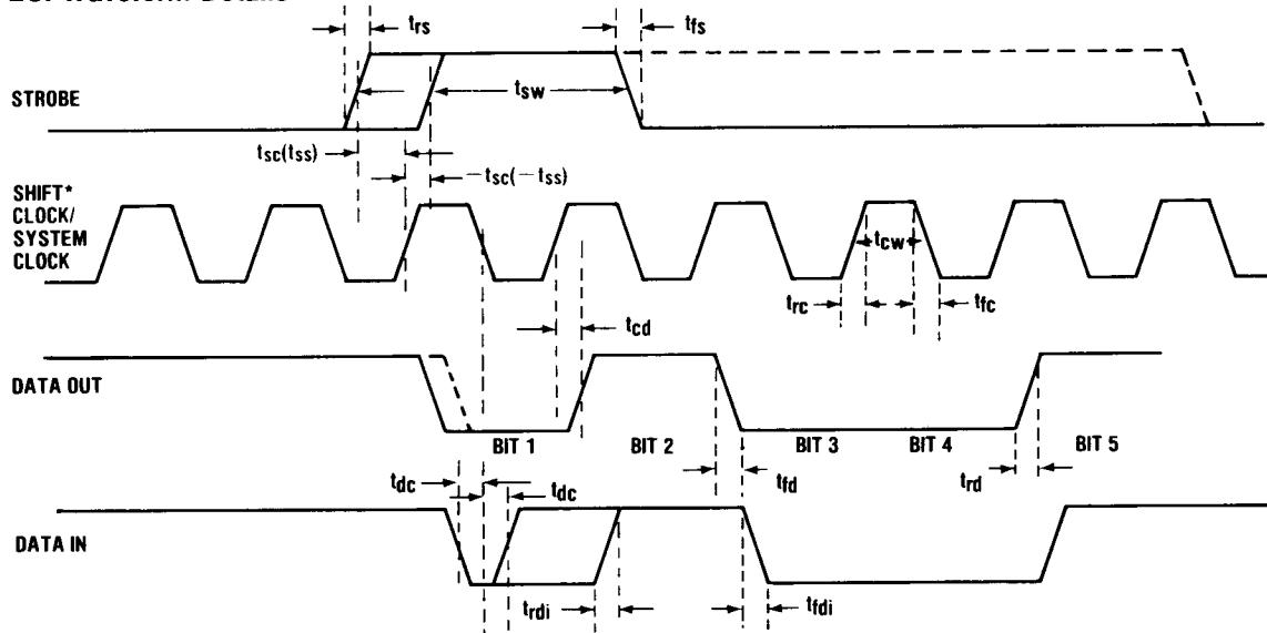
Figure 2C. Waveform Details
