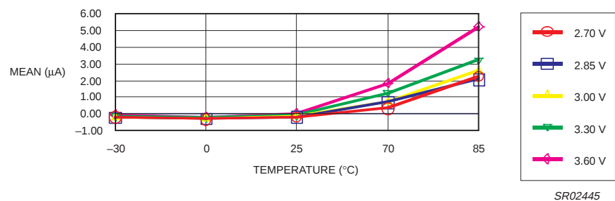
Figure 25. Total sleep I_{CC} .
