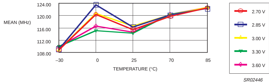
Figure 26. VCO 0011 bandwidth.
