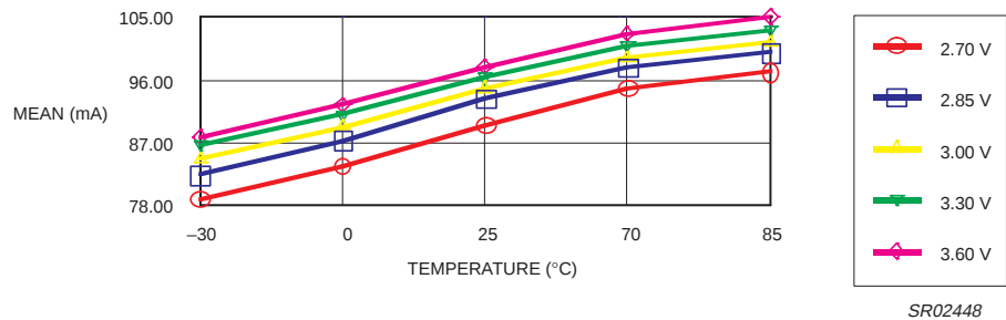
Figure 28. Total TX LOW I_{CC} .
