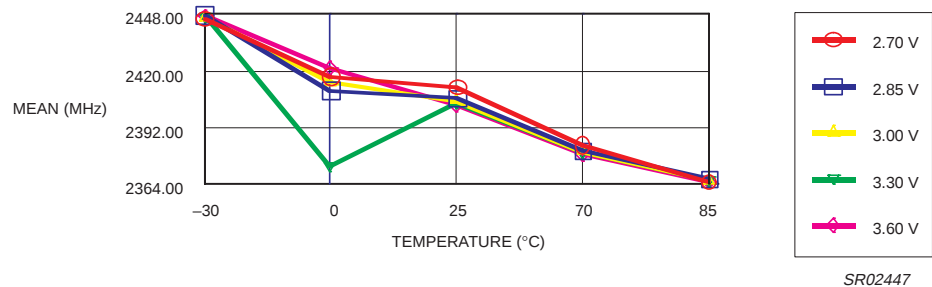
Figure 27. VCO 0111 f_1 .
