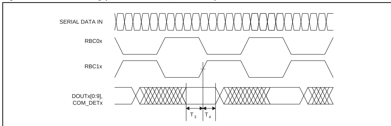
Figure 14. Receiver Timing (Full Clock Mode, CMODE = 1)
