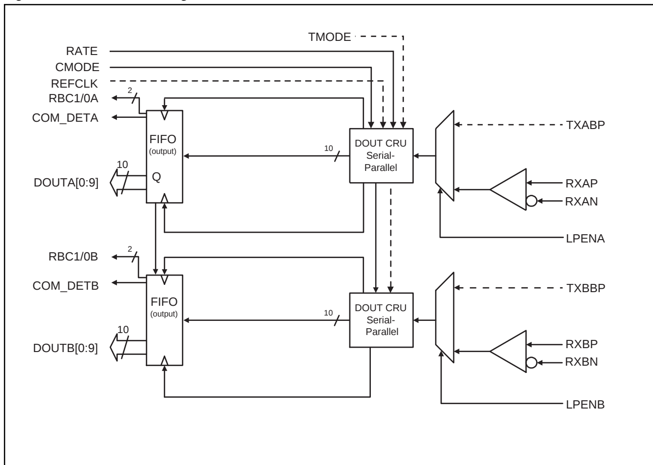
Figure 4. Receiver Block Diagram
