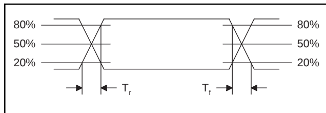
Figure 18. Serial Input/Output Rise and Fall Time
