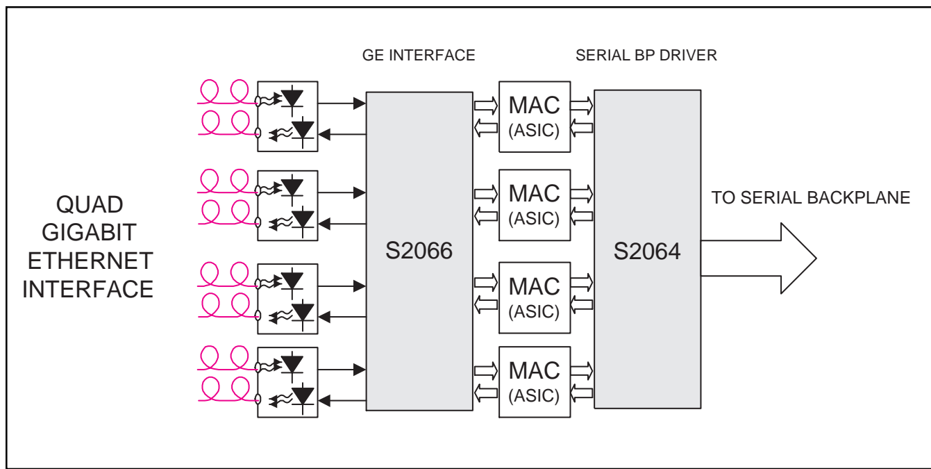
Figure 1. Typical Quad Gigabit Ethernet Application
