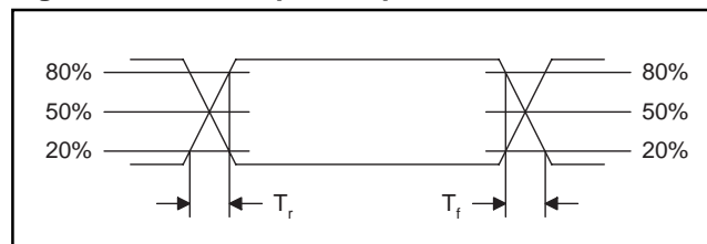
Figure 19. Serial Input/Output Rise and Fall Time
