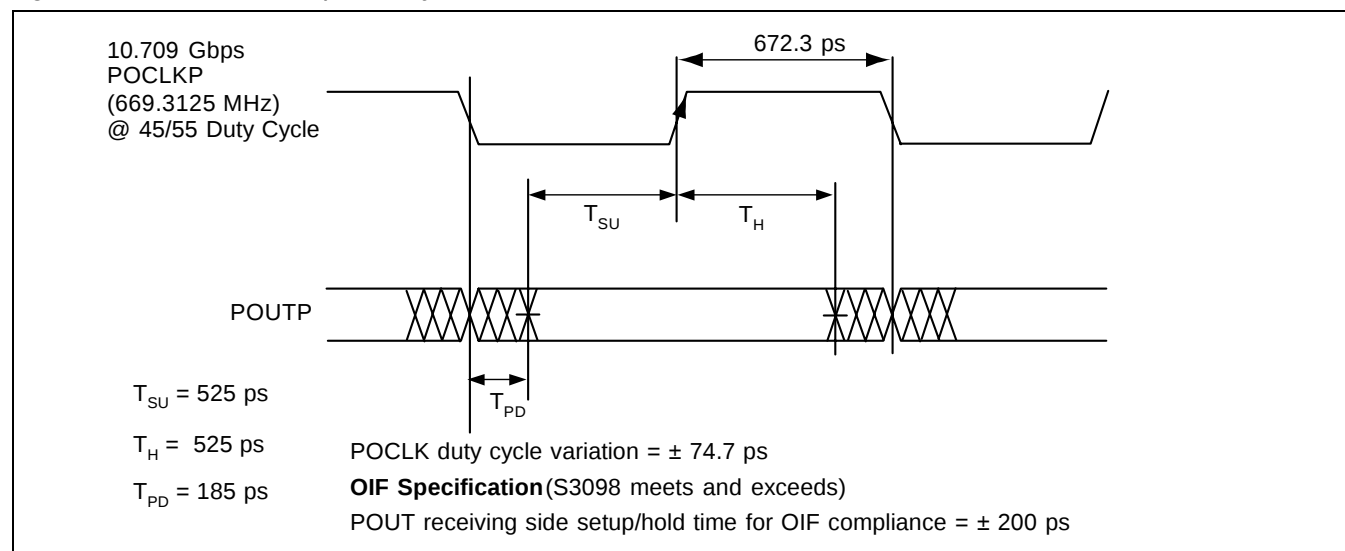
Figure 5. Parallel Data Output Delay from POCLK 1,2
