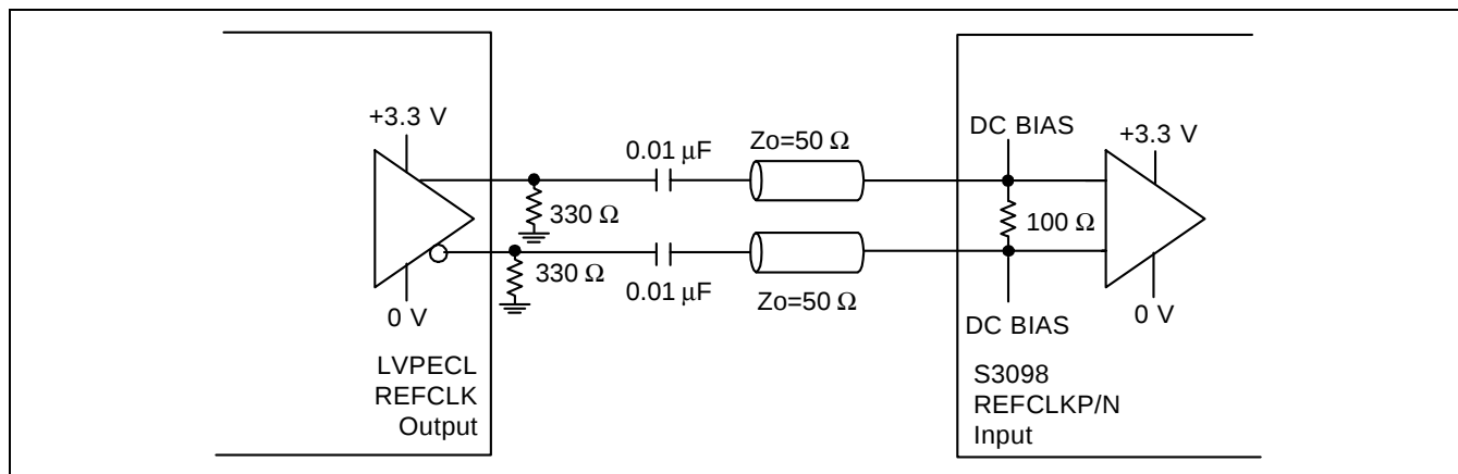
Figure 11. +3.3 V Differential LVPECL Driver to S3098 LVPECL Reference Clock Input, AC Coupled Termination
