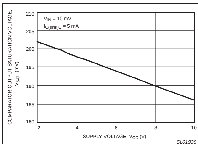
Figure 26. Comparator output saturation voltage versus supply voltage.
