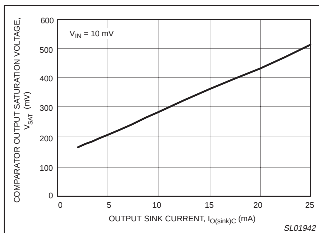
Figure 30. Comparator output saturation voltage versus sink current.
