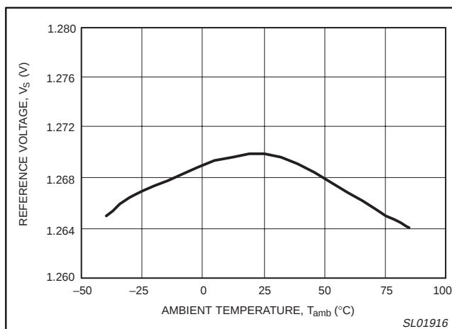
Figure 4. Reference voltage versus ambient temperature.
