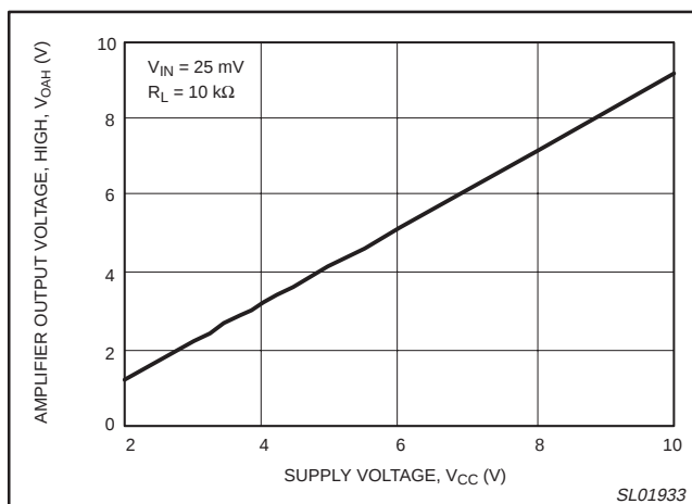
Figure 22. Amplifier output voltage, HIGH versus supply voltage.
