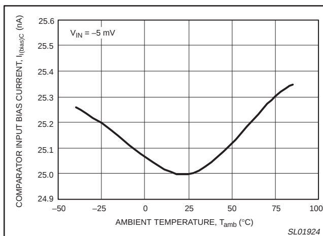
Figure 12. Comparator bias current versus ambient temperature.
