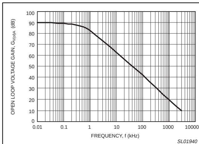
Figure 28. Amplifier open loop gain versus frequency.
