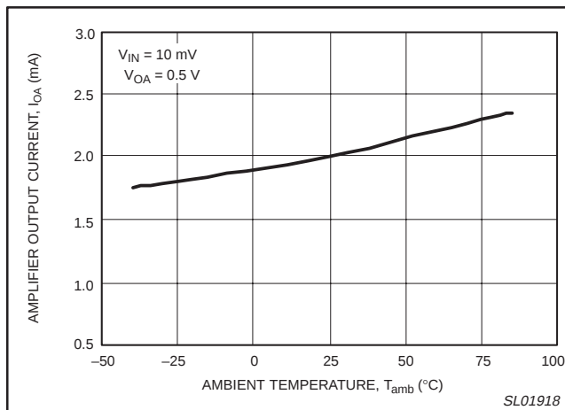
Figure 8. Amplifier output current versus ambient temperature.
