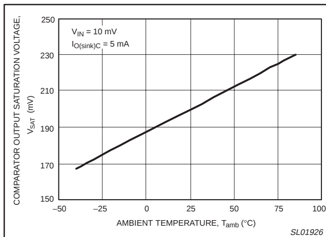
Figure 14. Comparator output saturation voltage versus ambient temperature.
