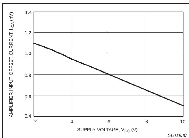
Figure 18. Amplifier input offset current versus supply voltage.
