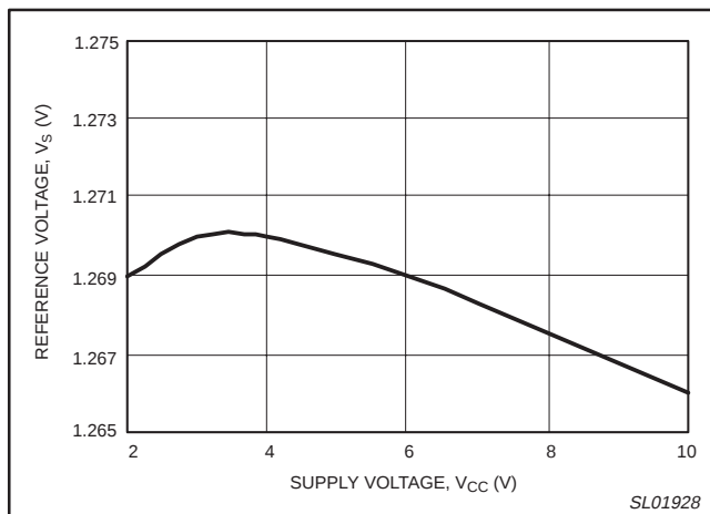
Figure 16. Reference voltage versus supply voltage.
