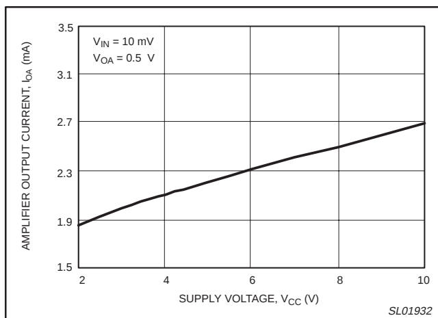
Figure 20. Amplifier output current versus supply voltage.
