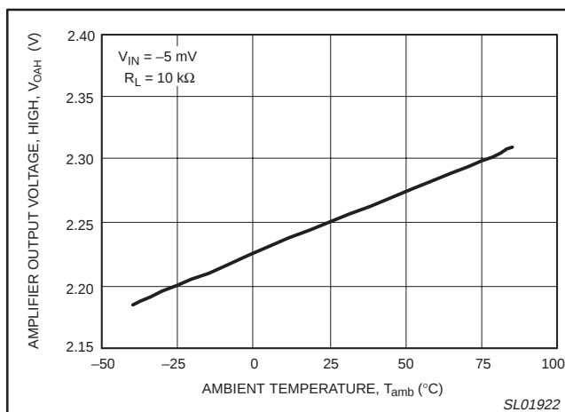
Figure 10. Amplifier output voltage, HIGH versus ambient temperature.
