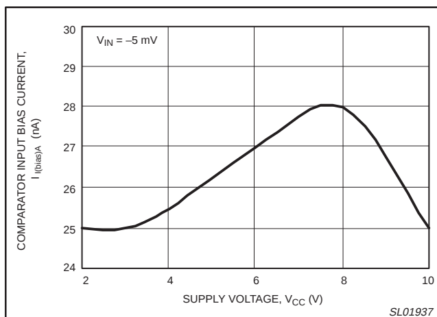
Figure 24. Comparator bias current versus supply voltage.
