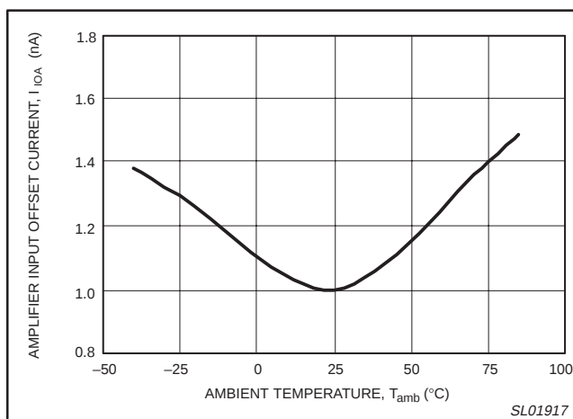
Figure 6. Amplifier input offset current versus ambient temperature.
