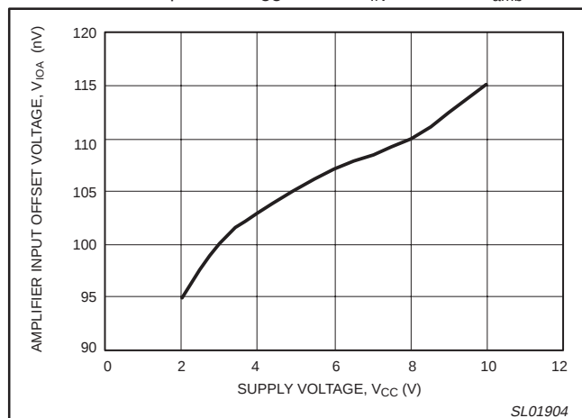
Figure 9. Amplifier input offset voltage versus supply voltage.
