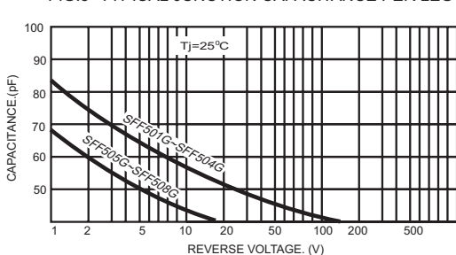
FIG. 5- TYPICAL JUNCTION CAPACITANCE PER LEG
