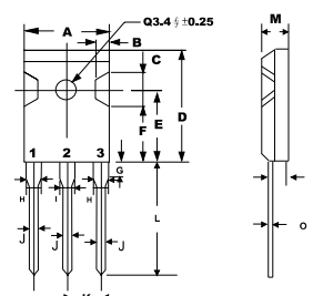
TO-247 (3P)
