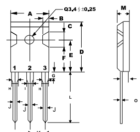
TO-247 (3P)
