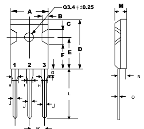
TO-247 (3P)
