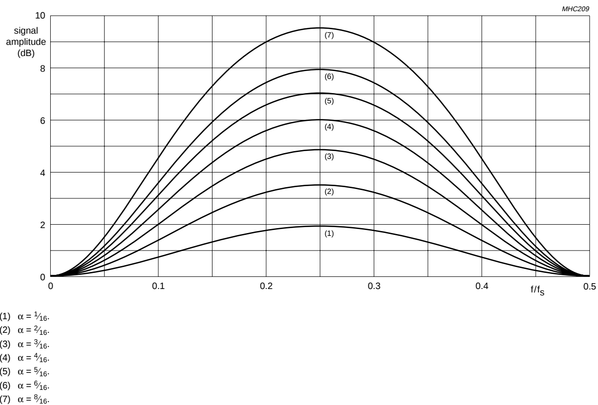
Fig.14 Transfer function of the peaking band-pass with variation of \alpha ( \beta = 0 ; \tau = 0 ).
