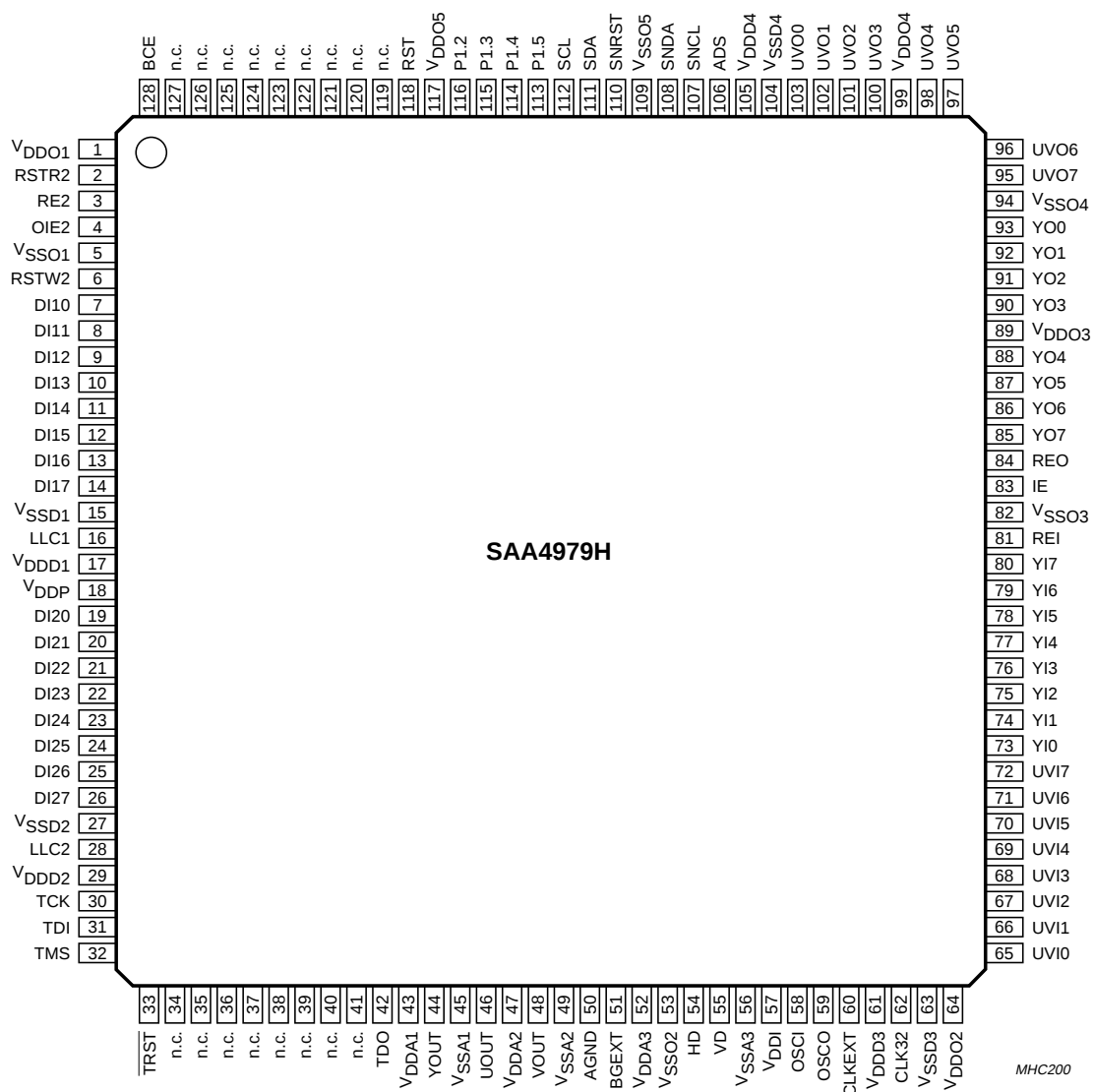
Fig.2 Pin configuration.
