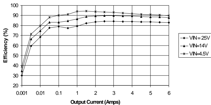
SC1485EVB Efficiency at V_{out} = 1.8V
