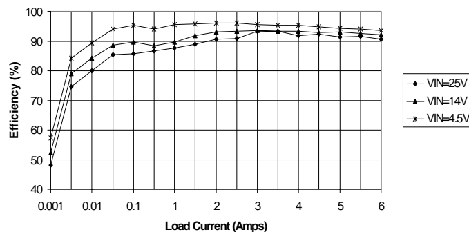
SC1485 Efficiency at V_{out} = 3.3V
