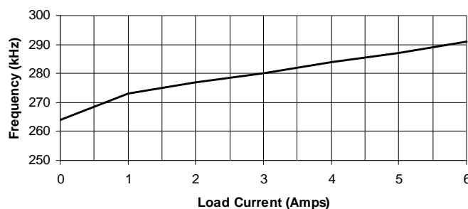
Frequency vs Load Current (V in = 15V, V out = 2.5V, R ton = 1M)
