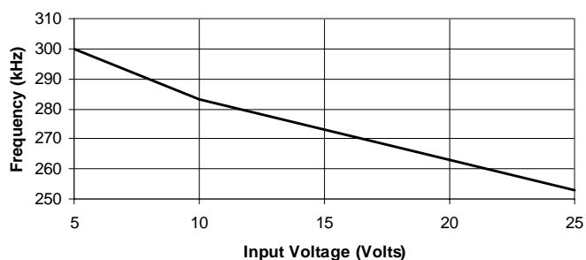
Frequency vs Input Voltage (I out = 1A, V out = 2.5V, R ton = 1M)
