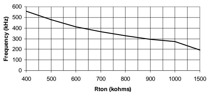
R ton vs Frequency (V in = 15V, V out = 2.5V, I out = 1A)
