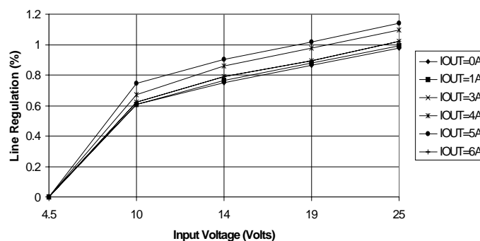
SC1485 Line Regulation at V_{out} = 3.3V
