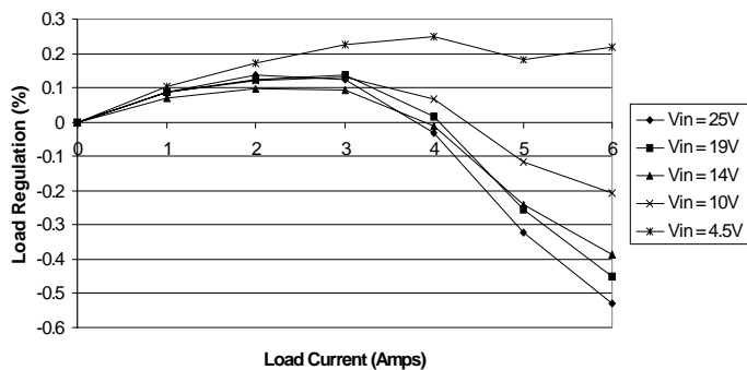
SC1485EVB Load Regulation at V_{out} = 1.8V
