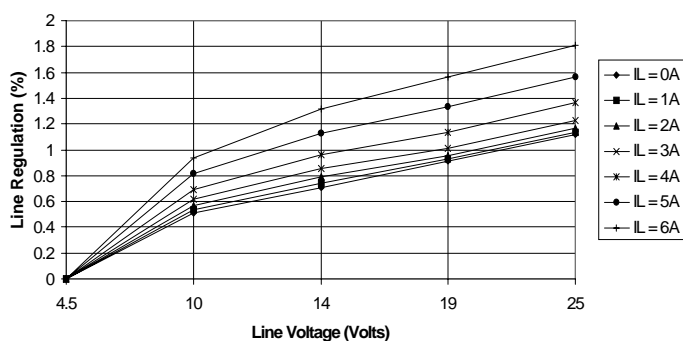
SC1485EVB Line Regulation at V_{out} = 1.8V
