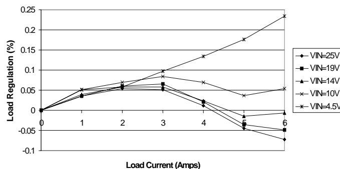
SC1485 Load Regulation at V_{out} = 3.3V
