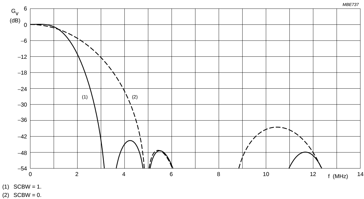
Fig.3 Chrominance transfer characteristic 1.
