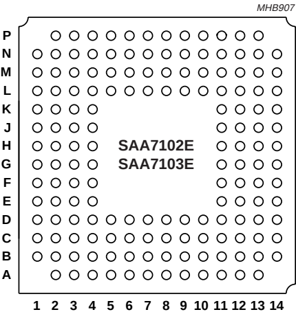
Fig.2 Pin configuration (SAA7102E; SAA7103E).
