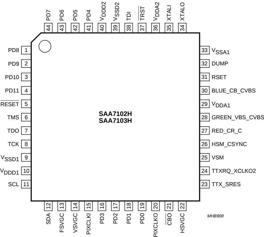
Fig.3 Pin configuration (SAA7102H; SAA7103H).
