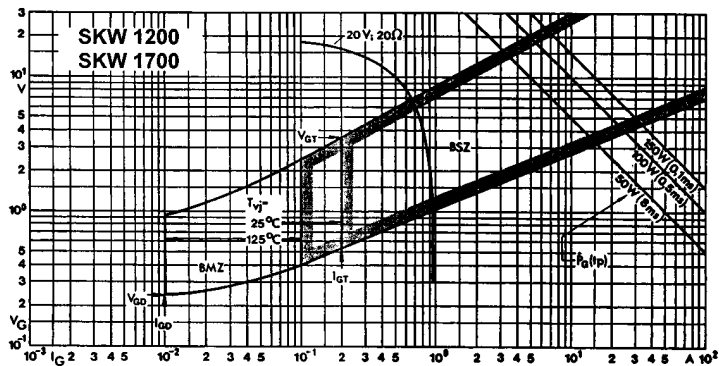
Fig. 8 Gate trigger characteristics
