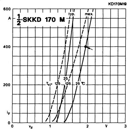
Fig. 19 Forward characteristics
