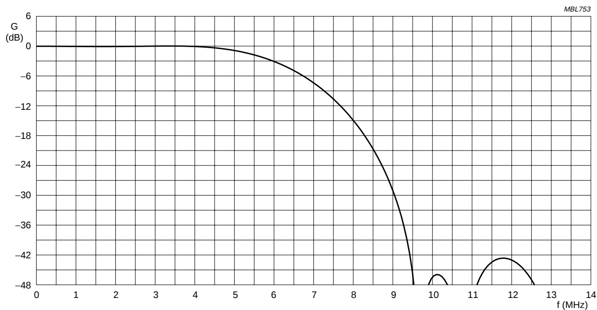
Fig.4 Decimation filter.
