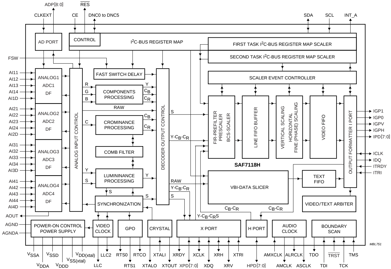
Fig.1 Block diagram.
