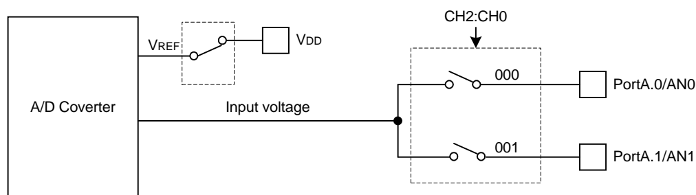
Figure 1 A/D Converter Block Diagram
