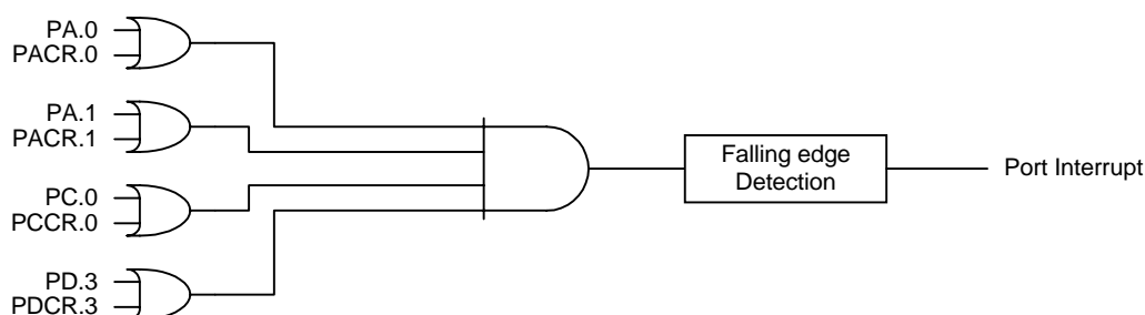
Figure 6 Port Interrupt function block-diagram
