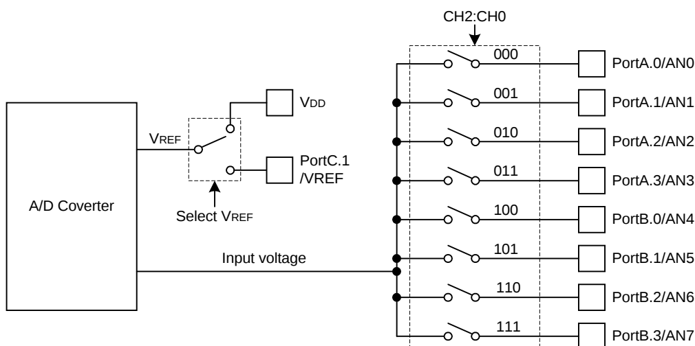
Figure 1 A/D Converter Block Diagram
