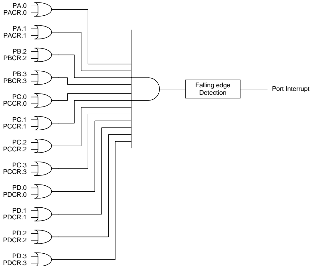
Figure 6 Port Interrupt function block-diagram
