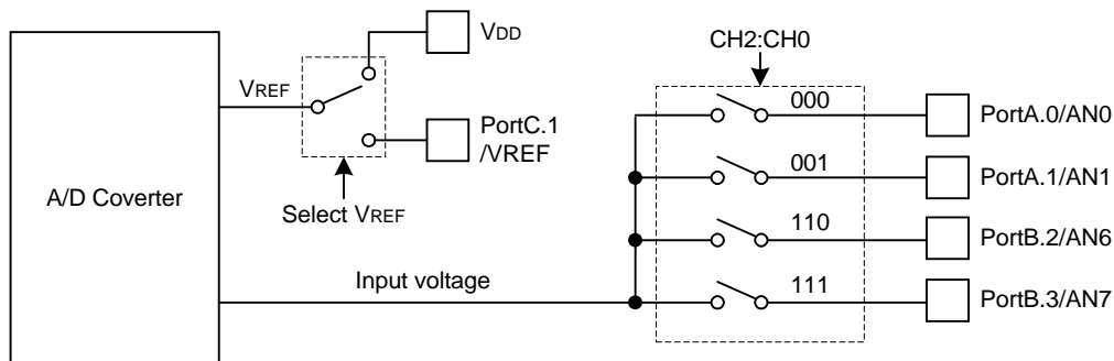
Figure 1 A/D Converter Block Diagram
