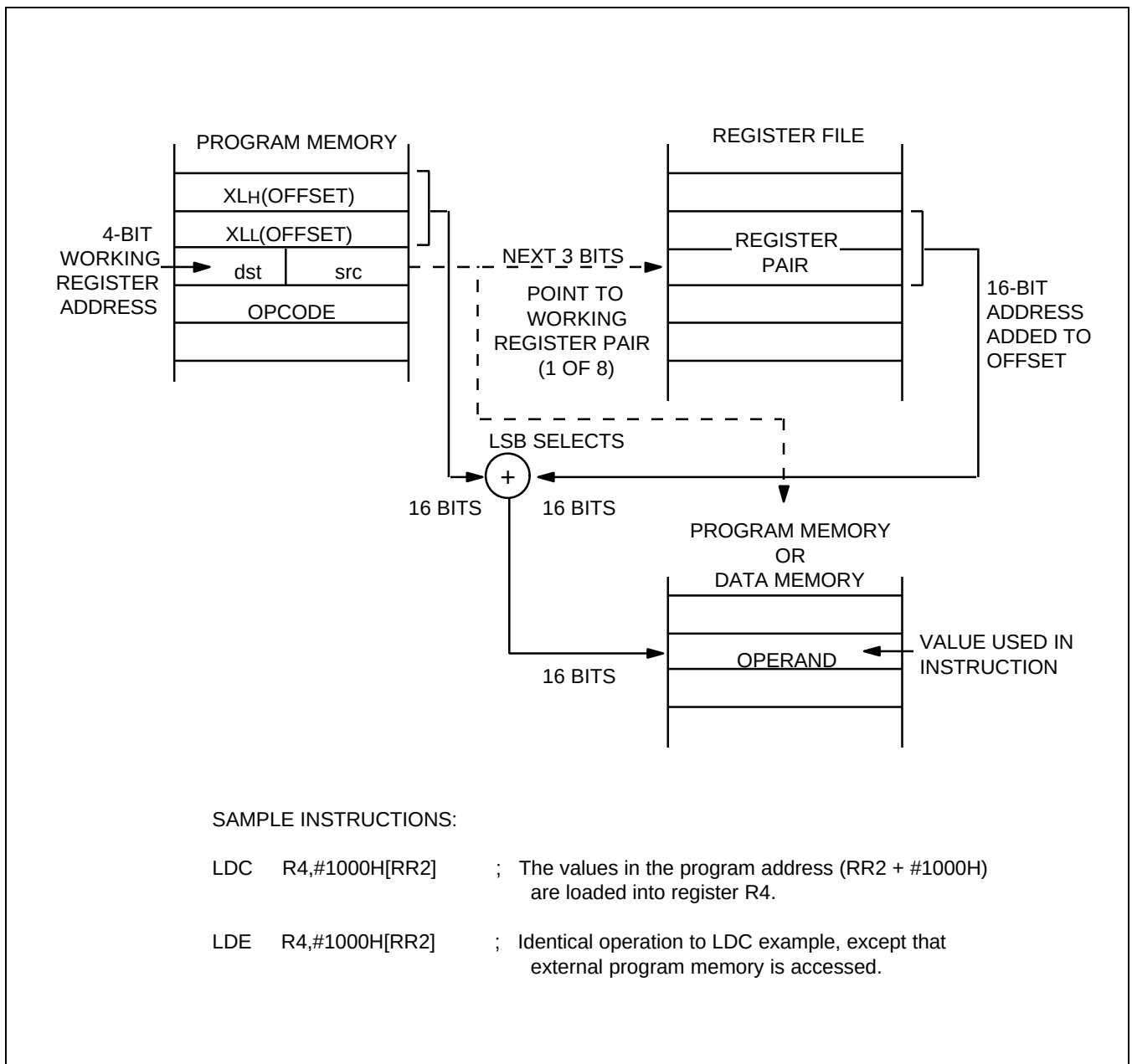
Figure 3-9. Indexed Addressing to Program or Data Memory with Long Offset
