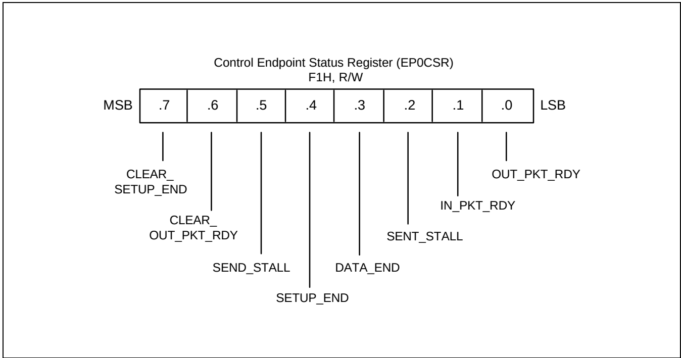
Figure 11-3. Control Endpoint Status Register (EP0CSR)
