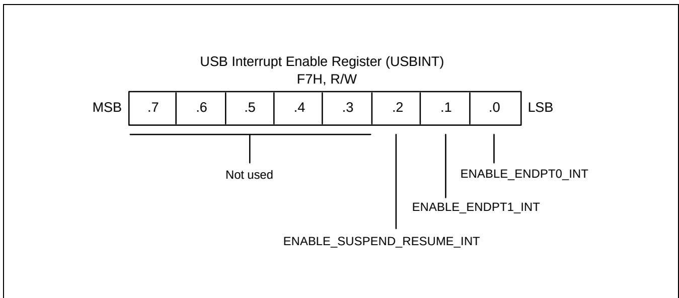
Figure 11-6. USB Interrupt Enable Register (USBINT)
