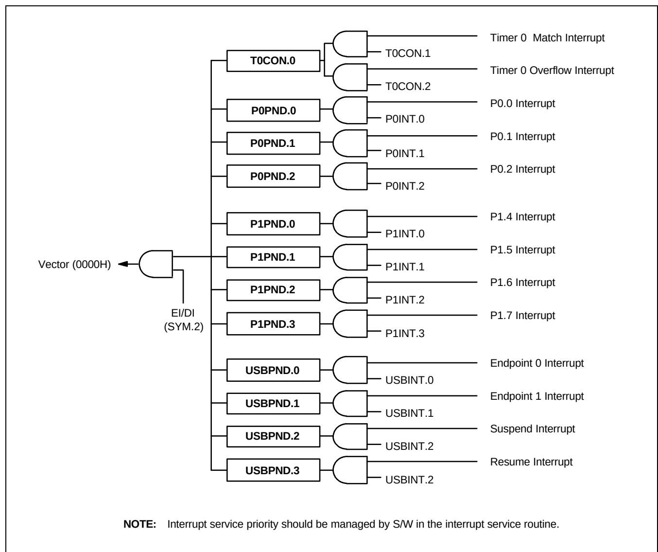
Figure 5-3. S3C9614/P9614 Interrupt Structure
