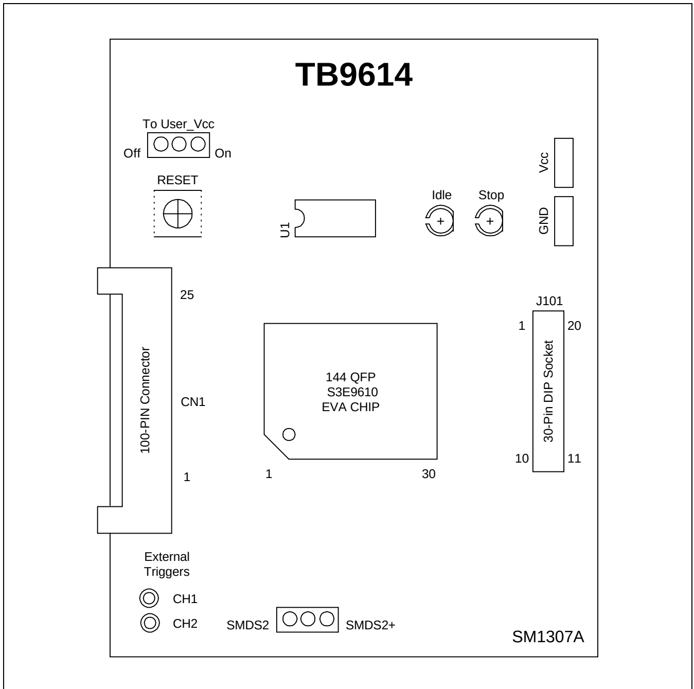
Figure 16-2. TB9614 Target Board Configuration
