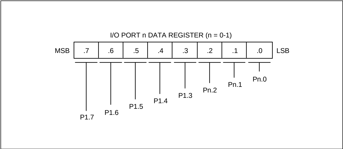
Figure 9-1. Port Data Register Format
