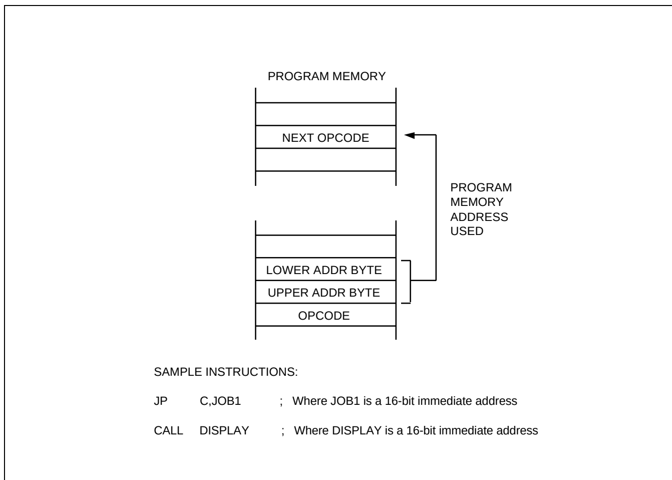
Figure 3-11. Direct Addressing for Call and Jump Instructions
