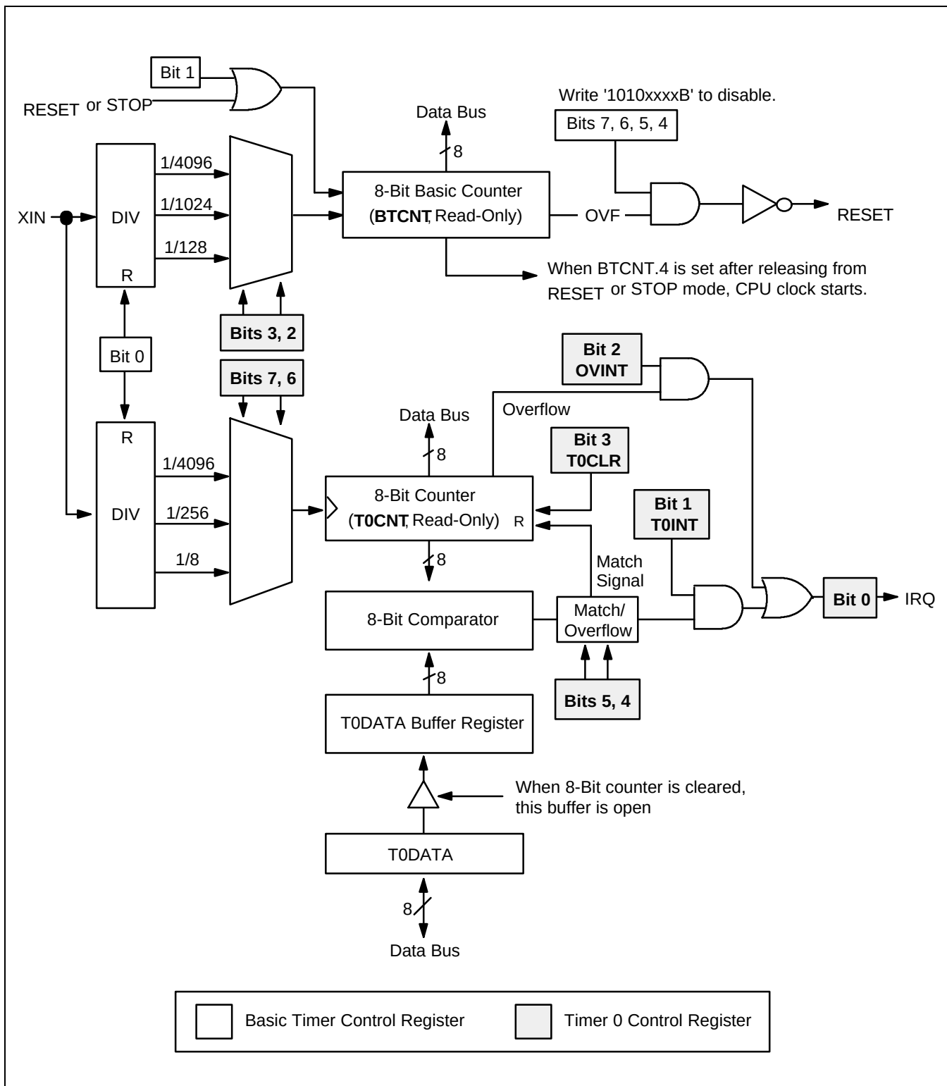
Figure 10-6. Basic Timer and Timer 0 Block Diagram
