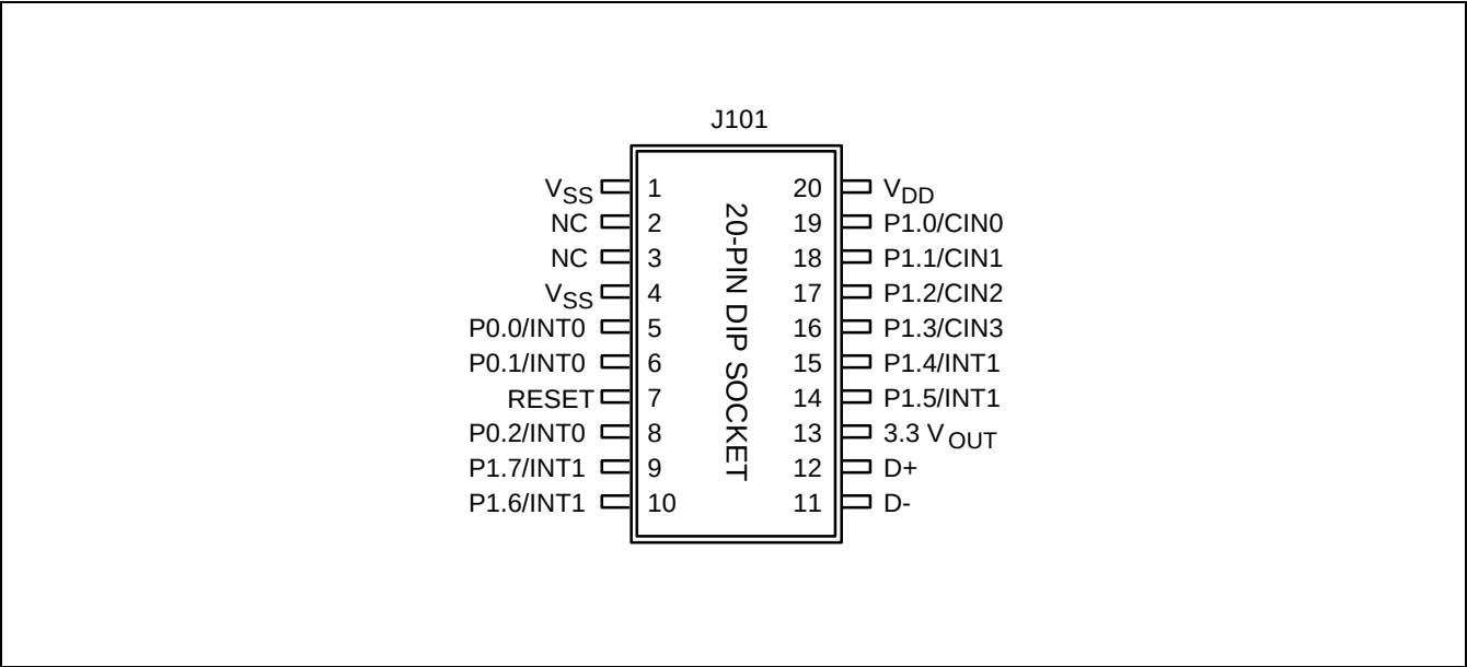
Figure 16-3. 20-Pin DIP Socket for TB9614
