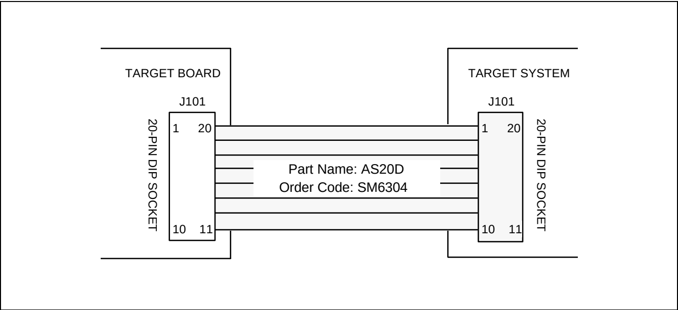
Figure 16-4. S3C9614 Probe Adapter Cable for 20-DIP Package
