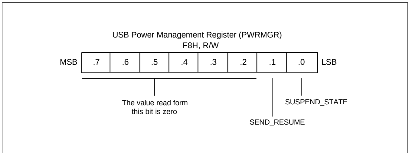
Figure 11-7. USB Power Management Register (PWRMGR)
