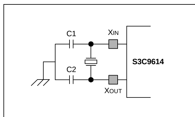
Figure 7-2. Main Oscillator Circuit (Crystal/Ceramic Oscillator)
