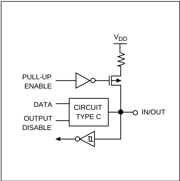
Figure 1-5. Pin Circuit Type D
