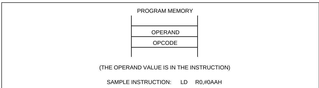
Figure 3-13. Immediate Addressing
