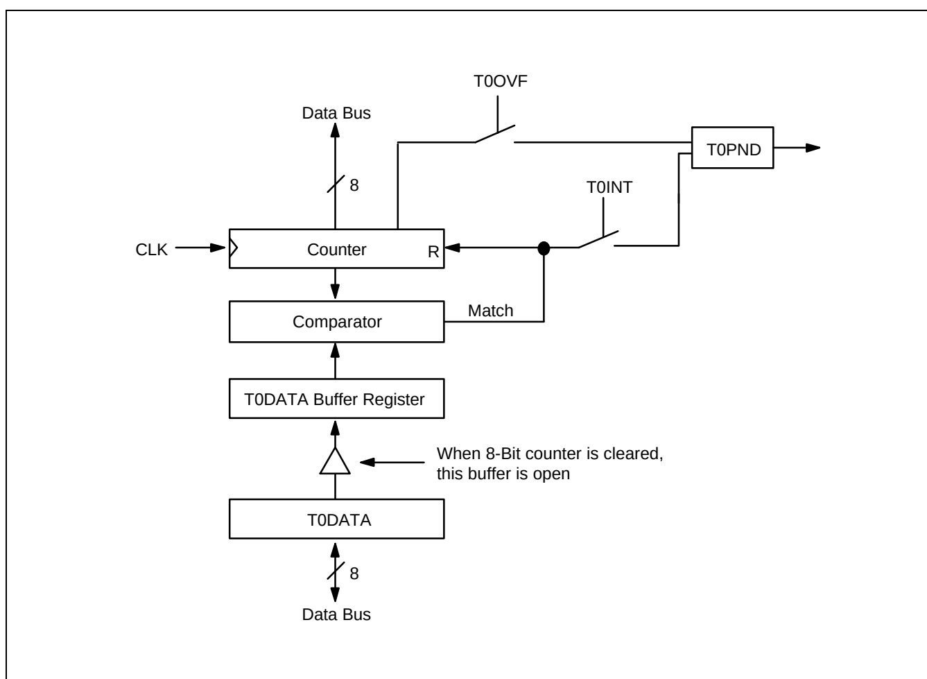
Figure 10-5. Simplified Timer 0 Function Diagram: Interval Timer Mode
