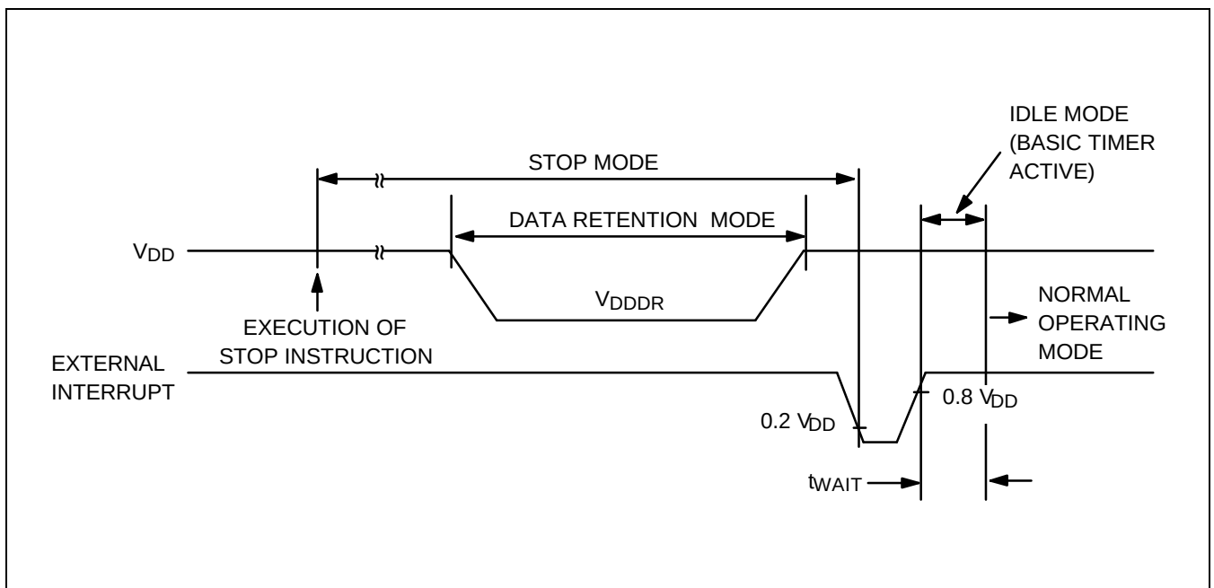
Figure 13-4. Stop Mode Release Timing When Initiated by an External Interrupt
