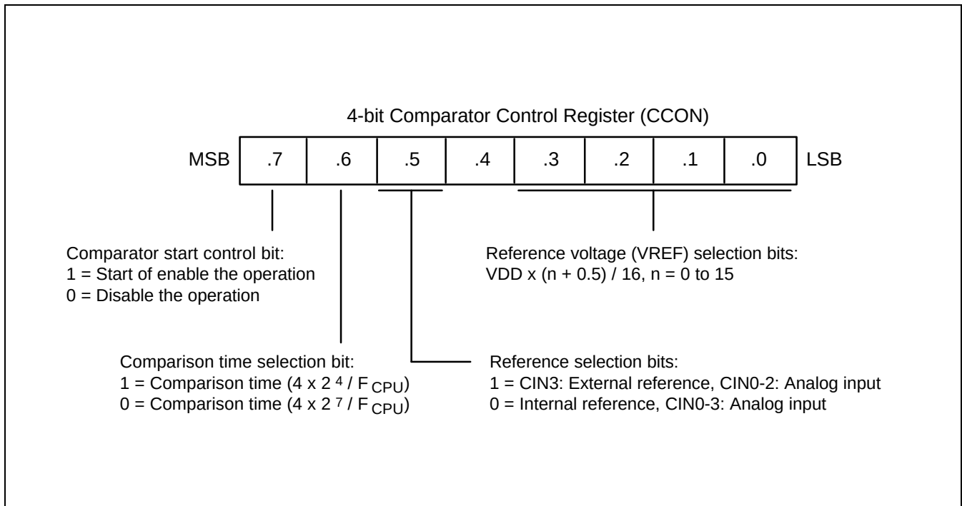
Figure 12-1. Comparison Control Register (CCON)
