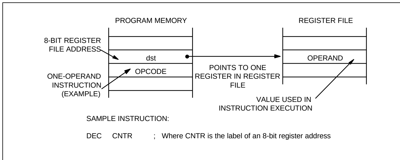
Figure 3-1. Register Addressing
