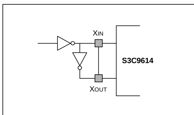
Figure 7-1. External Oscillator
