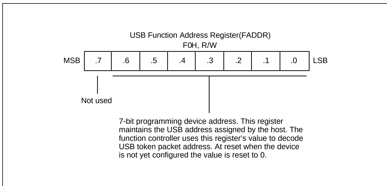
Figure 11-2. USB Function Address Register (FADDR)
