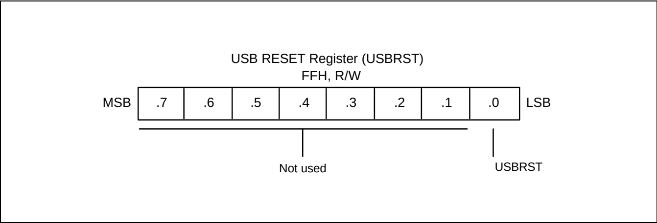
Figure 11-8. USB RESET Register (USBRST)
