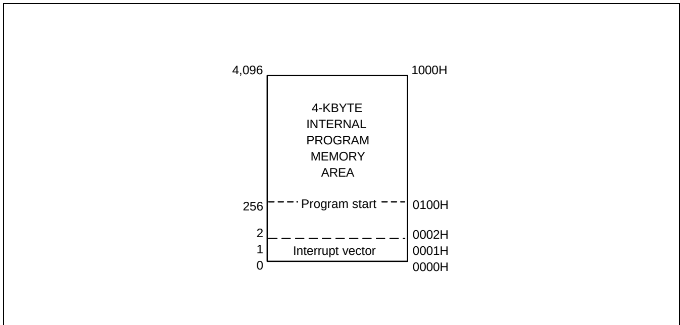
Figure 2-1. Program Memory Address Space
