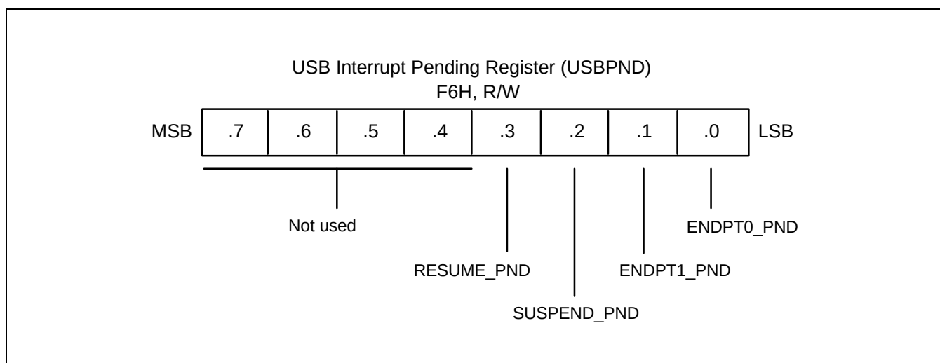
Figure 11-5. USB Interrupt Pending Register (USBPND)
