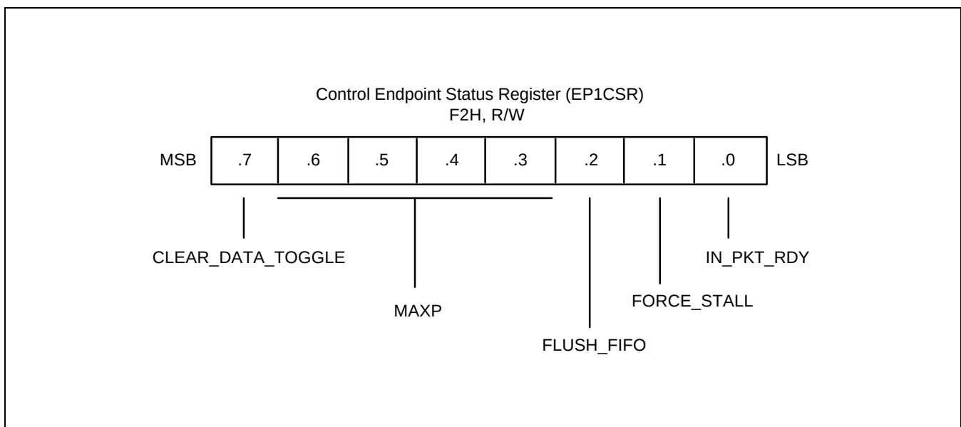
Figure 11-4. Interrupt Endpoint Status Register (EP1CSR)
