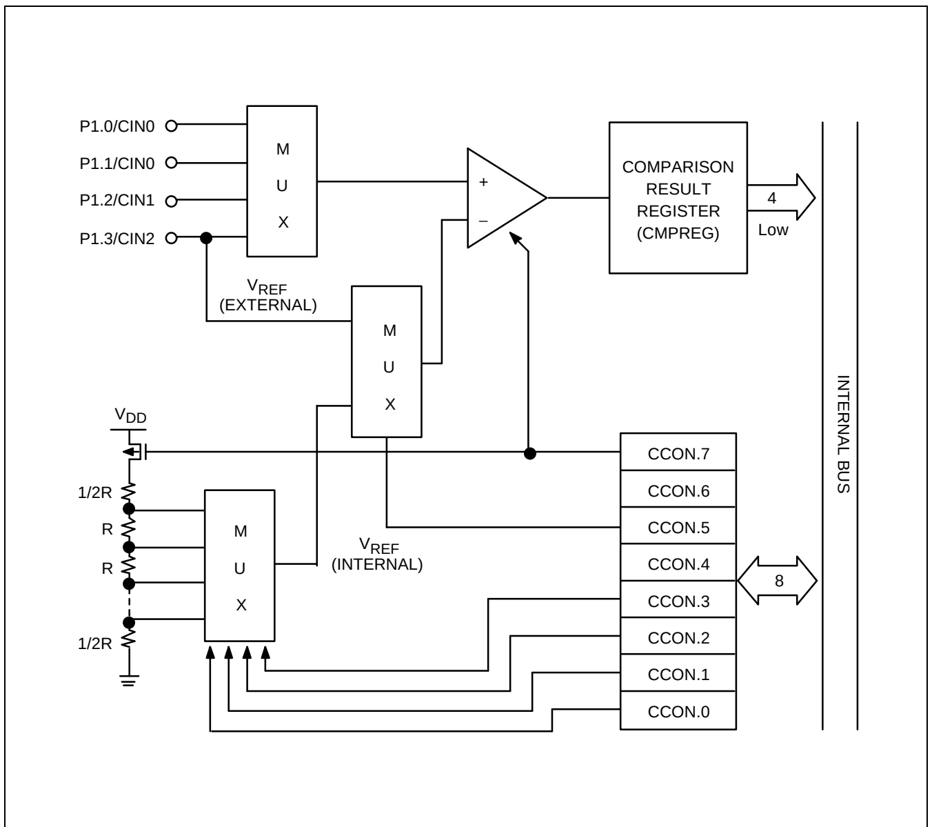
Figure 12-2. Comparator Functional Block Diagram
