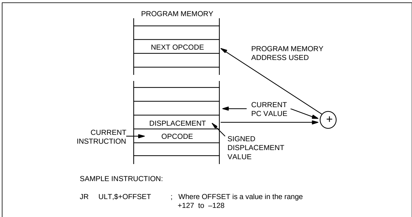
Figure 3-12. Relative Addressing
