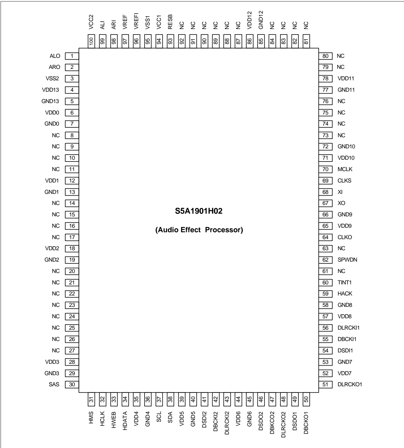
Figure 3. S5A1901H02 Pin Assignmen
