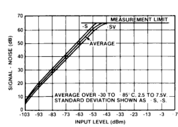
Fig. 14 Signal + noise to noise ratio vs input level
