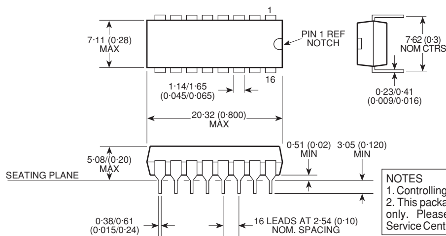
16-LEAD PLASTIC DIL – DP16
