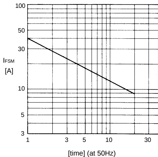
Surge capability
