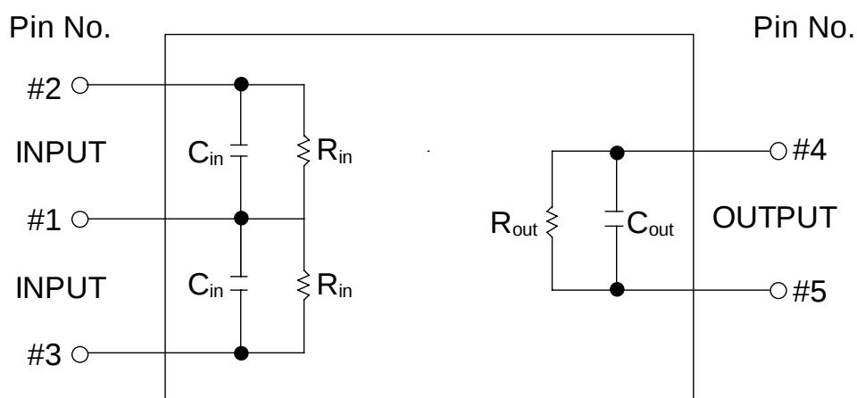
Fig.3 Equivalent circuit
