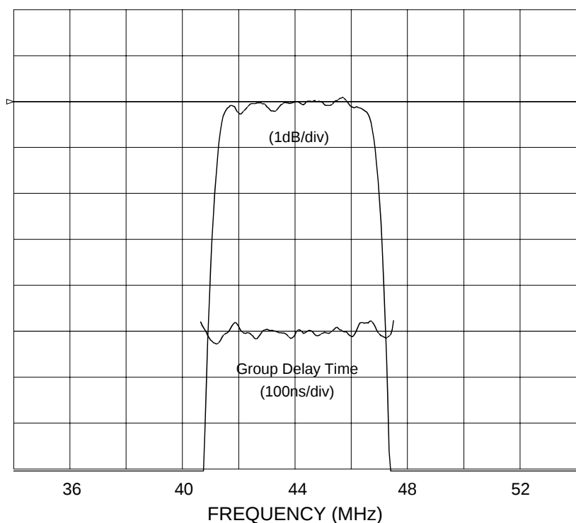
In-band Characteristics
