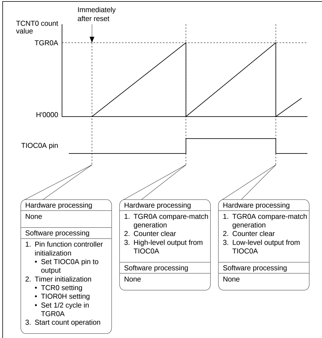
Figure 2-2-3 Principles of Pulse Output Operation
