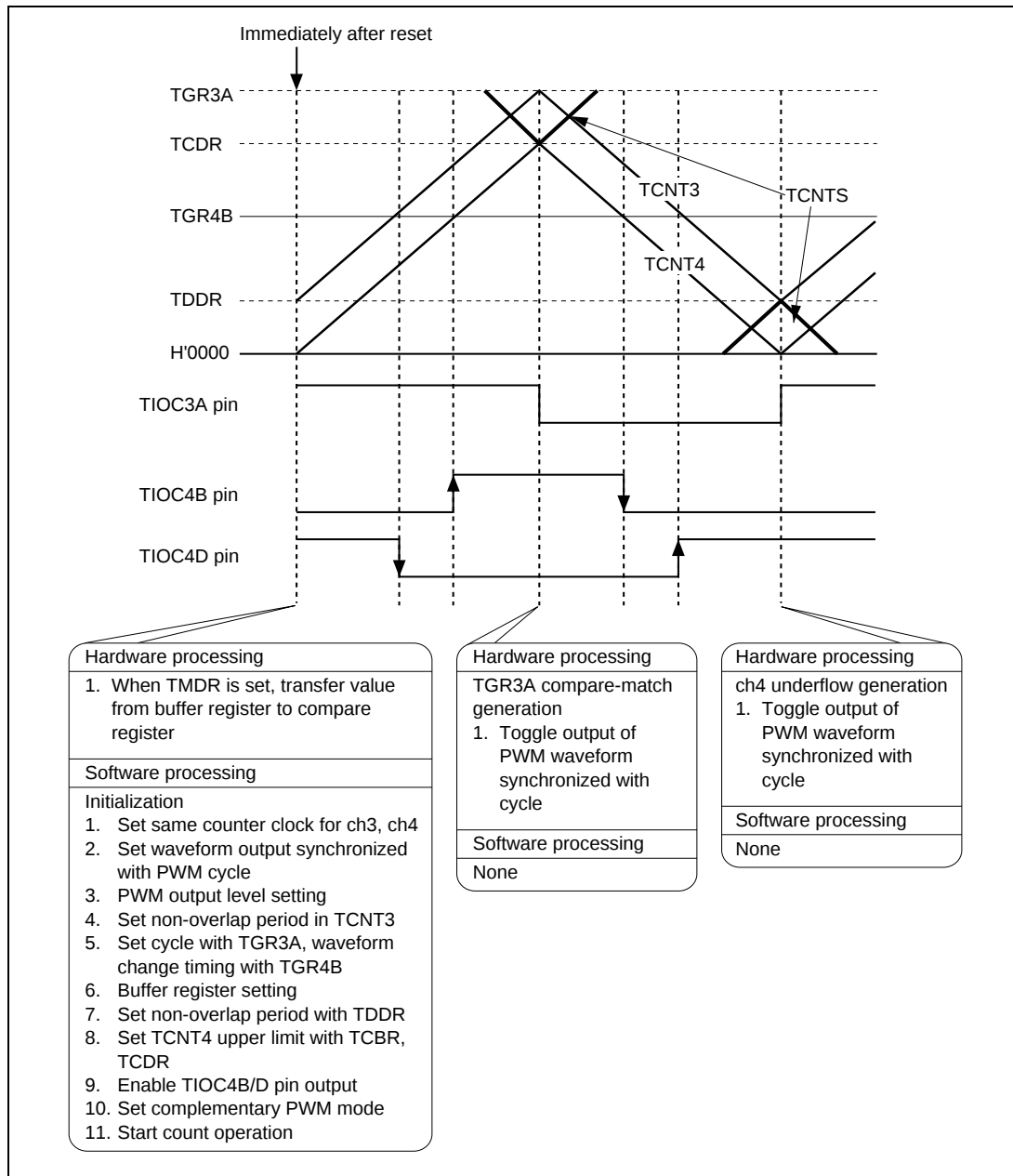
Figure 2-6-7 Principles of Toggle Waveform Output Operation Synchronized with PWM Cycle
