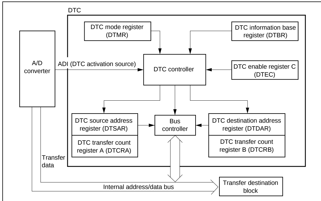
Figure 2-10-4 SH7040 DTC Block Diagram
