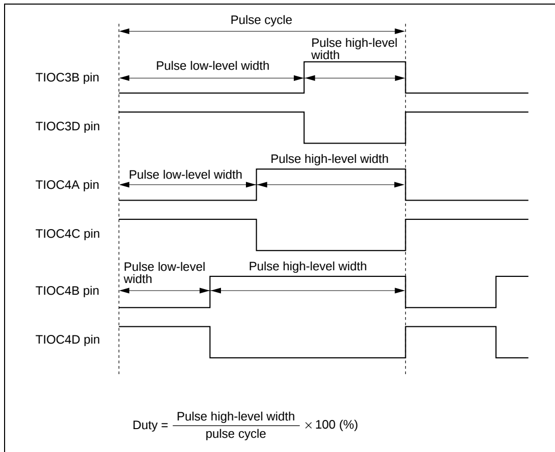
Figure 2-5-1 Example of Positive-Phase and Opposite-Phase PWM 3-Phase Output Waveform
