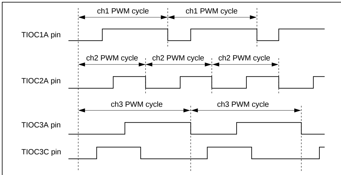
Figure 2-3-1 Example of PWM Output
