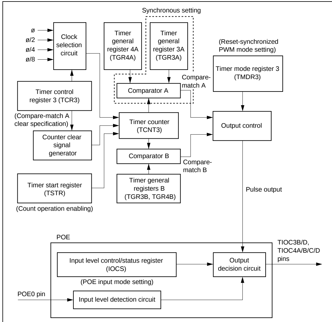
Figure 2-8-2 MTU/ch3, ch4, POE Block Diagram
