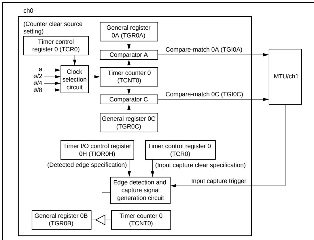
Figure 2-7-2 MTU/ch0 Block Diagram
