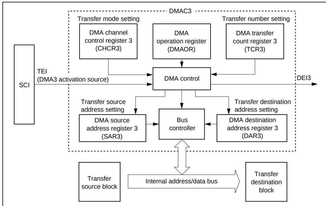
Figure 2-11-7 DMAC/ch3 Block Diagram
