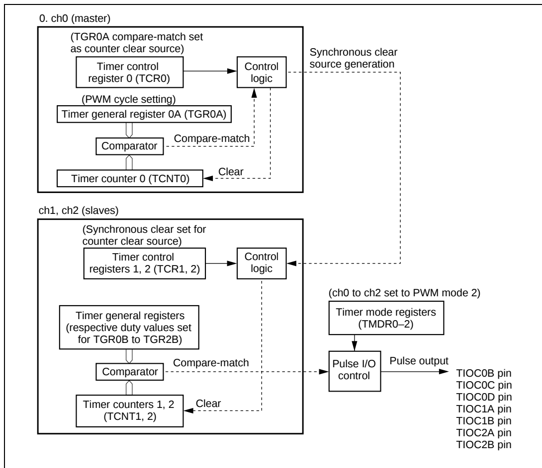
Figure 2-4-2 Synchronous Clear Block Diagram
