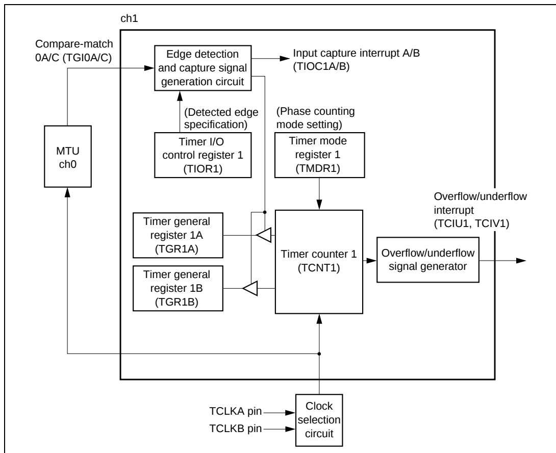
Figure 2-7-3 MTU/ch1 Block Diagram
