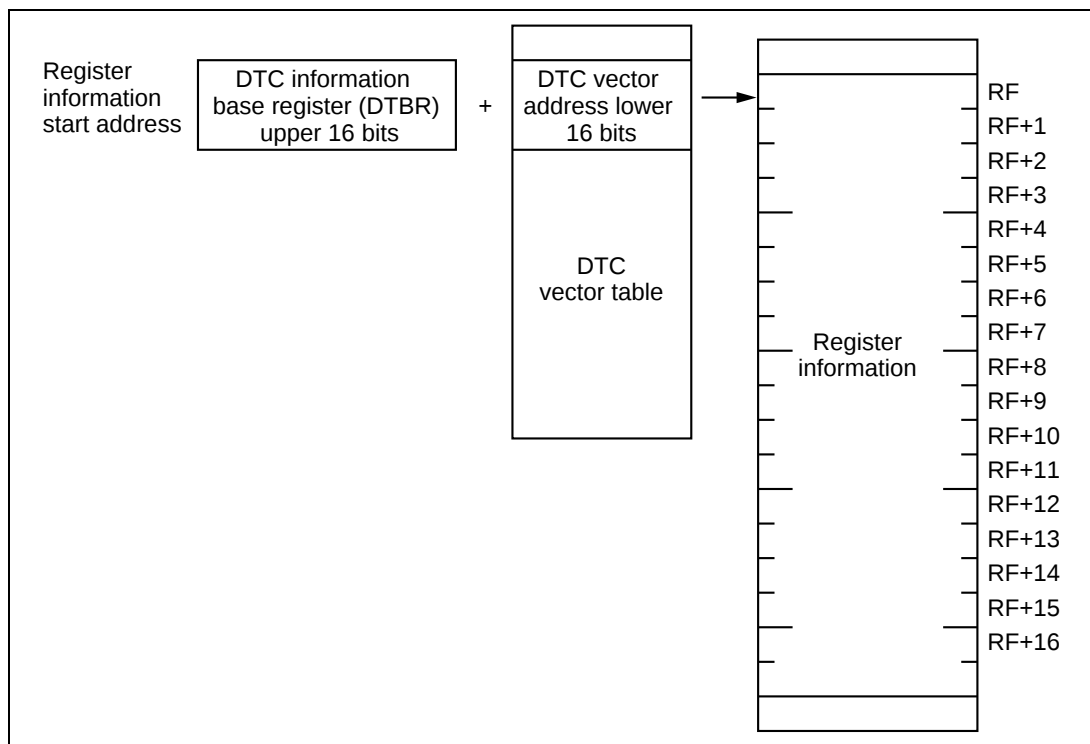
Figure 2-10-6 Principles of the DTC Activated Operation
