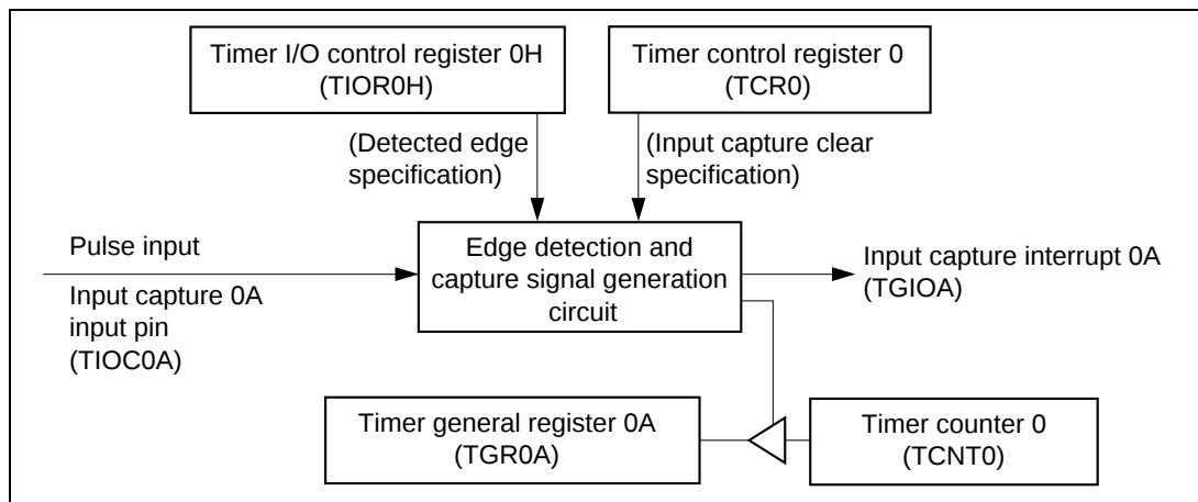
Figure 2-1-2 MTU/ch0 Block Diagram
