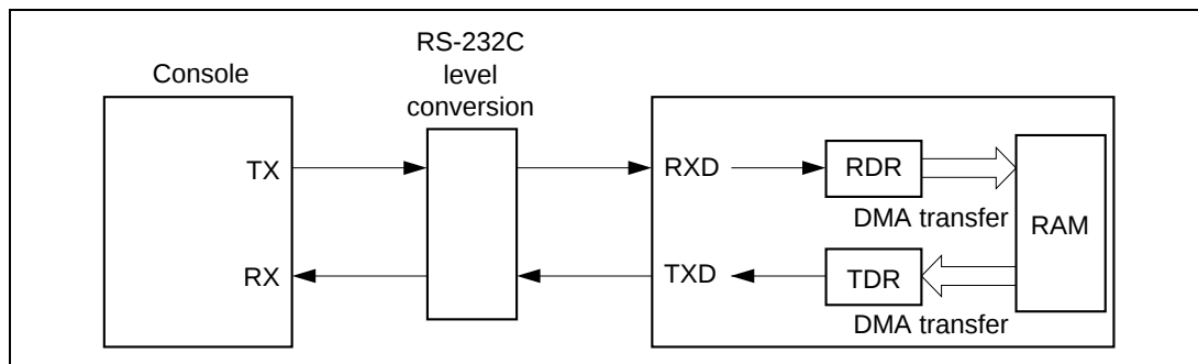
Figure 2-11-1 Block Diagram of SCI Transfer of RAM Data by SH7040
