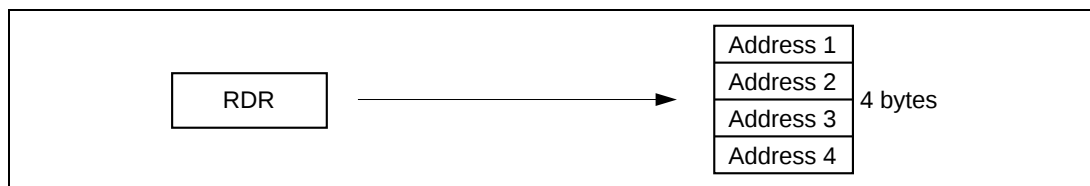
Figure 2-11-2 Data Transfer Using DMAC (Transfer Source Direct Address)
