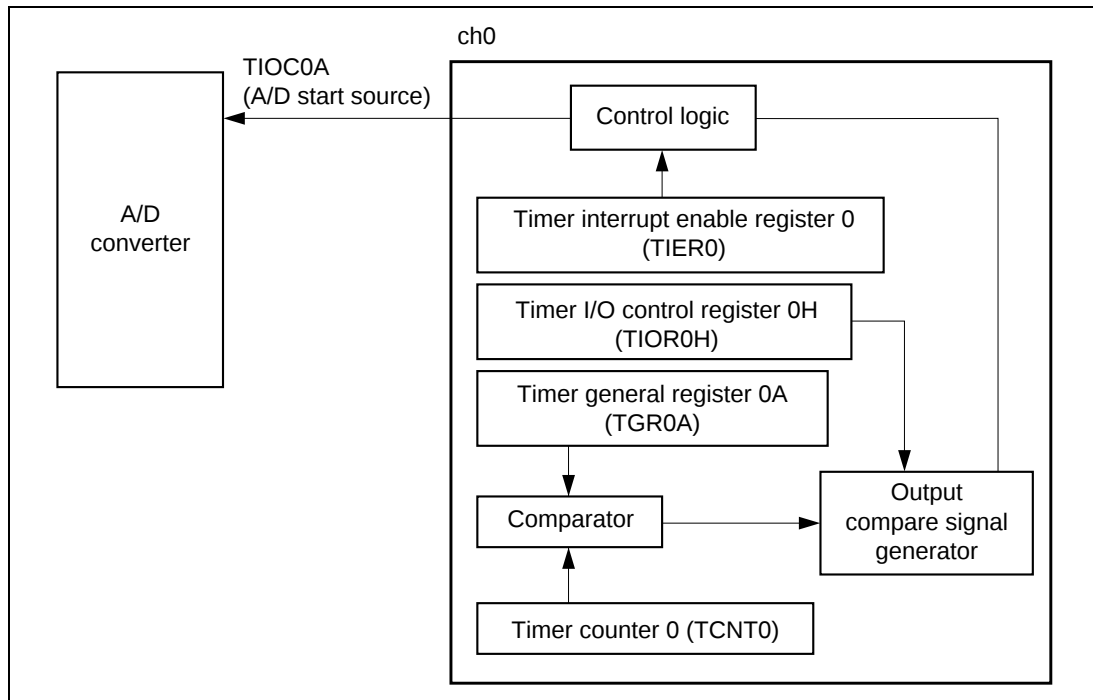
Figure 2-10-2 SH7040 ch0 Block Diagram
