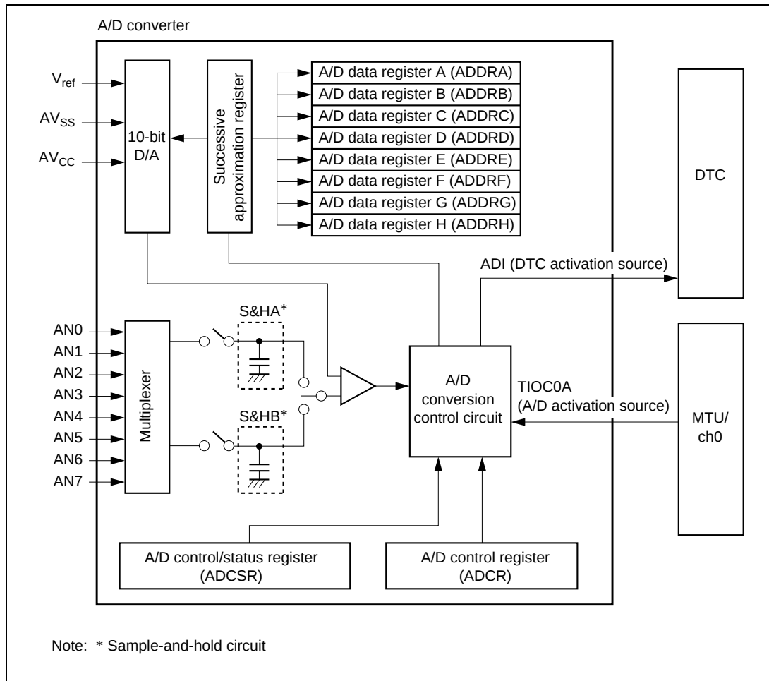
Figure 2-10-3 Block Diagram of Voltage Measurement by SH7040
