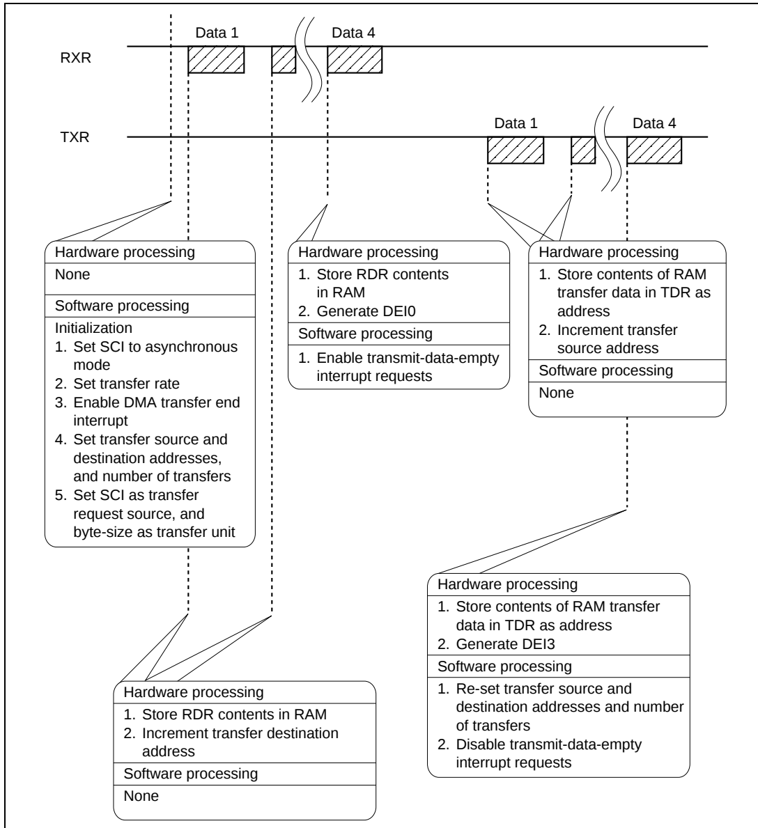
Figure 2-11-8 Principles of Data Transfer Operation Using SCI
