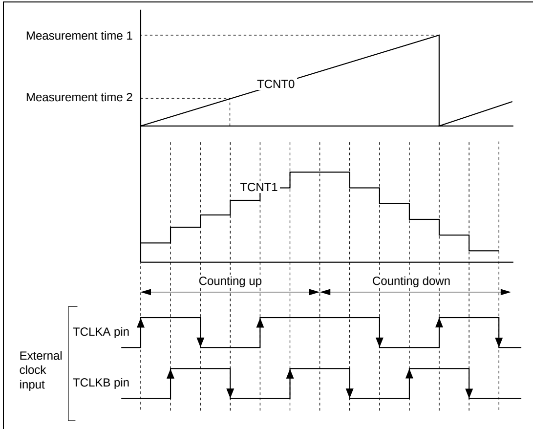
Figure 2-7-1 2-Phase Encoder Counter Latching
