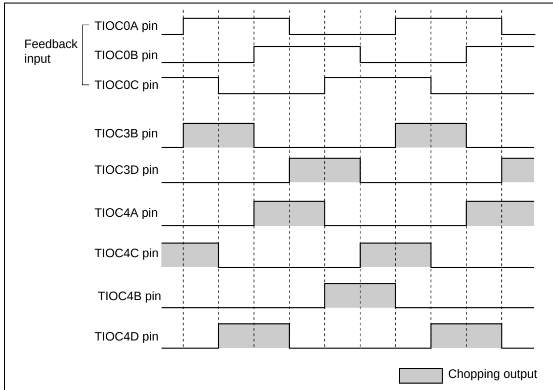
Figure 2-9-1 Example of DC Brushless Motor Control Signal Output
