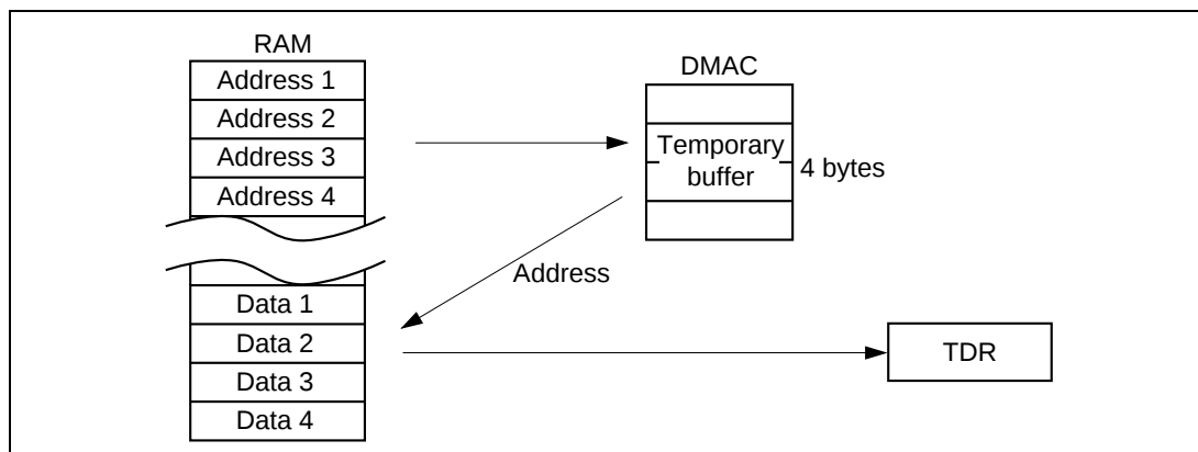
Figure 2-11-3 Data Transfer Using DMAC (Transfer Source Indirect Address)
