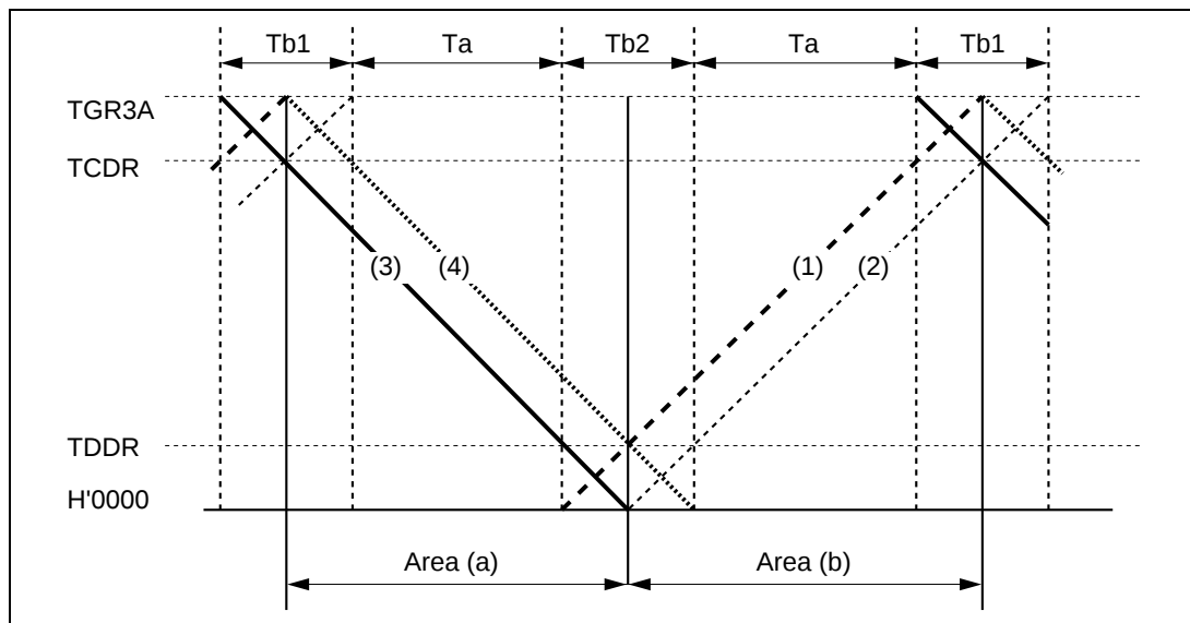
Figure 2-6-4 Principles of Operation of PWM Waveform Output Method
