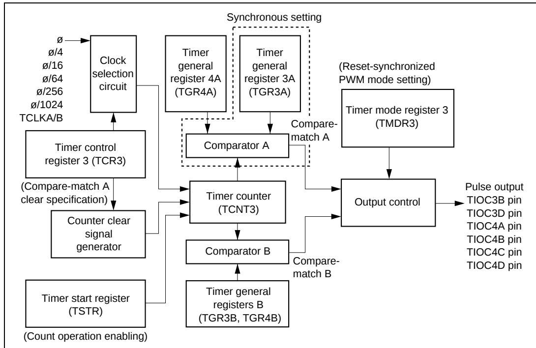
Figure 2-5-2 MTU/ch3, ch4 Block Diagram
