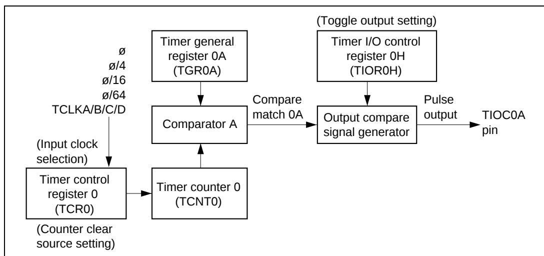
Figure 2-2-2 MTU/ch0 Block Diagram
