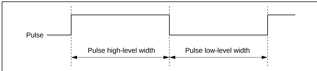
Figure 2-1-1 Pulse Width Measurement Timing
