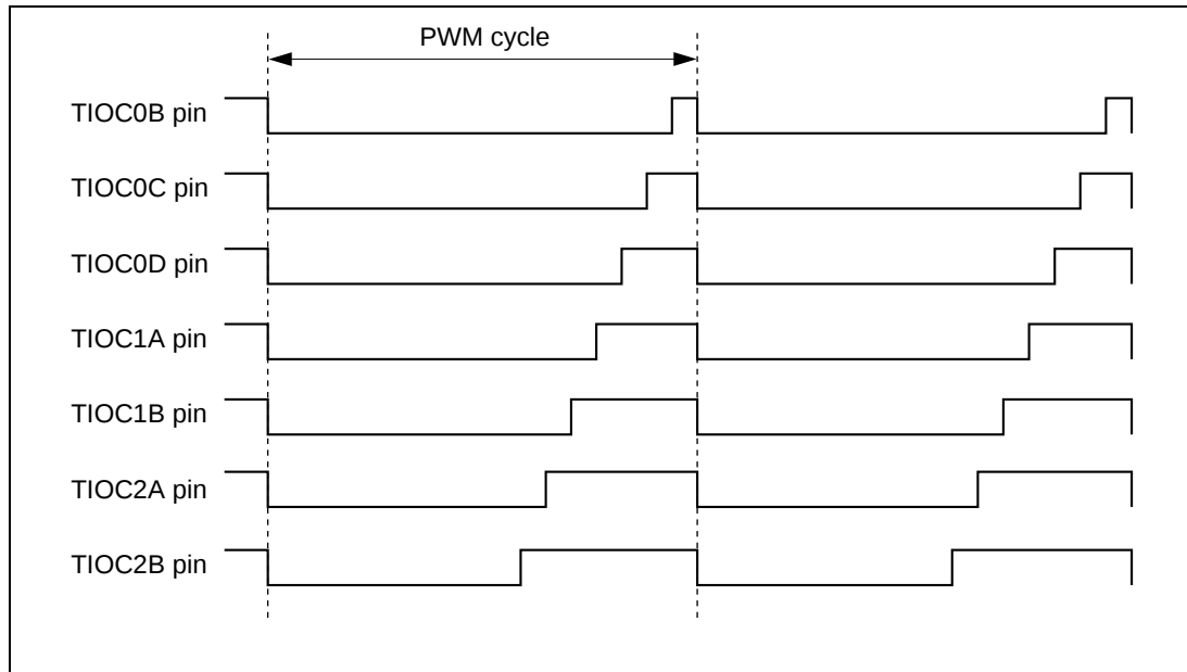
Figure 2-4-1 Example of PWM Output
