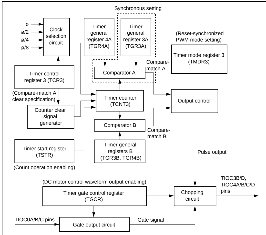
Figure 2-9-2 MTU/ch3, ch4 Block Diagram
