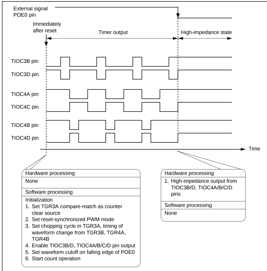
Figure 2-8-3 Principles of Externally Triggered Timer Waveform Cutoff Operation
