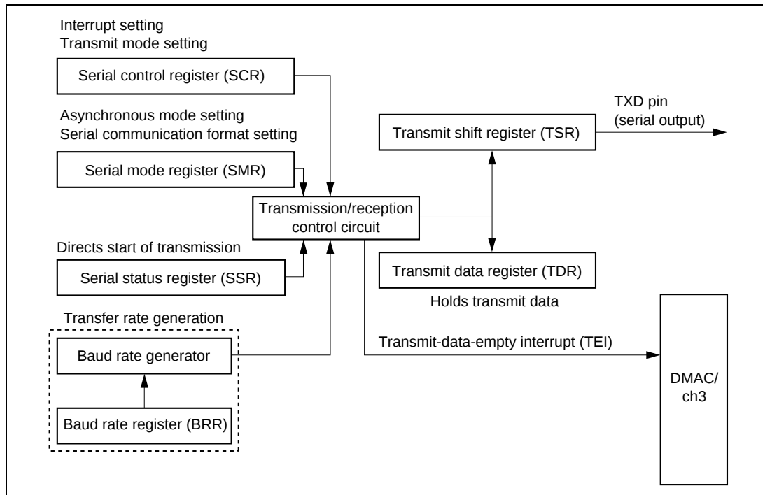
Figure 2-11-4 SCI Transmission Block Diagram
