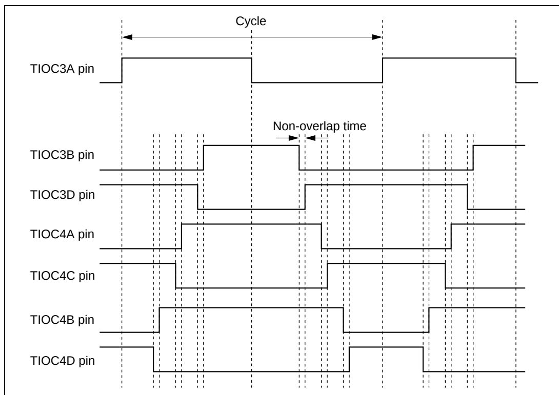
Figure 2-6-1 Complementary PWM 3-Phase Output Waveform
