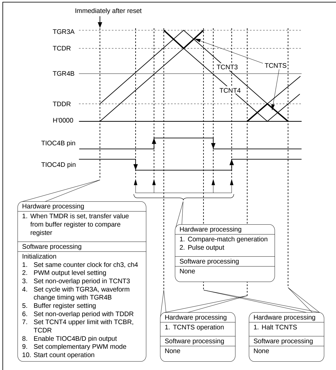
Figure 2-6-3 Principles of Complementary PWM Single-Phase Waveform Output Operation
