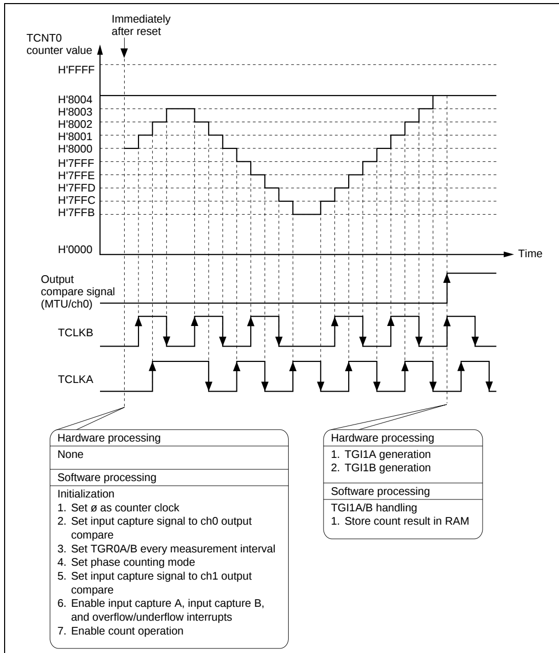
Figure 2-7-5 Principles of Phase Counting Mode Operation (2)
