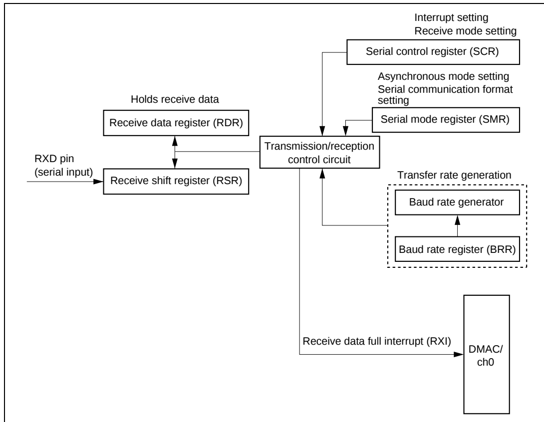
Figure 2-11-5 SCI Reception Block Diagram
