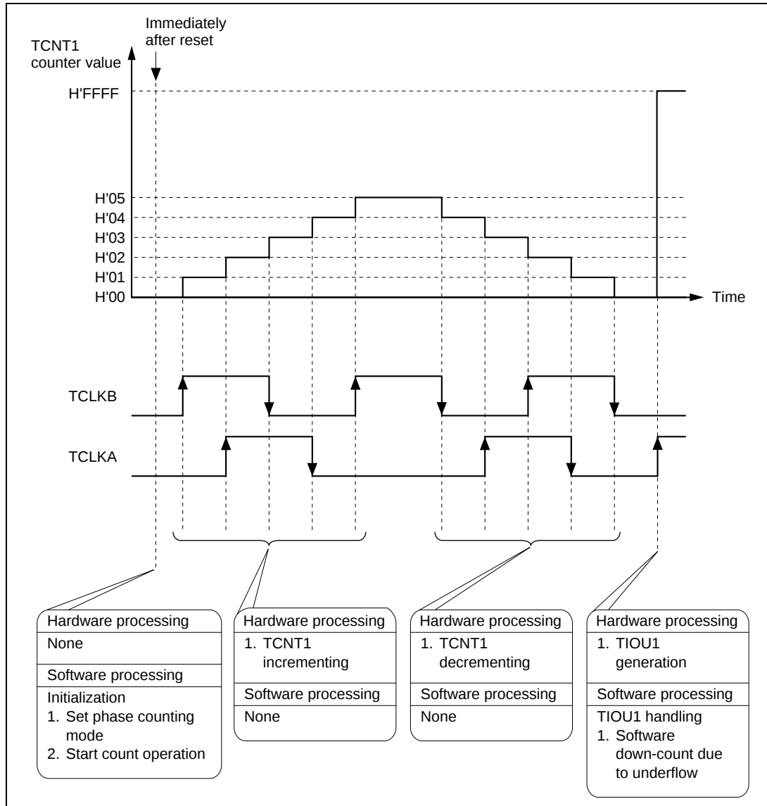
Figure 2-7-4 Principles of Phase Counting Mode Operation (1)
