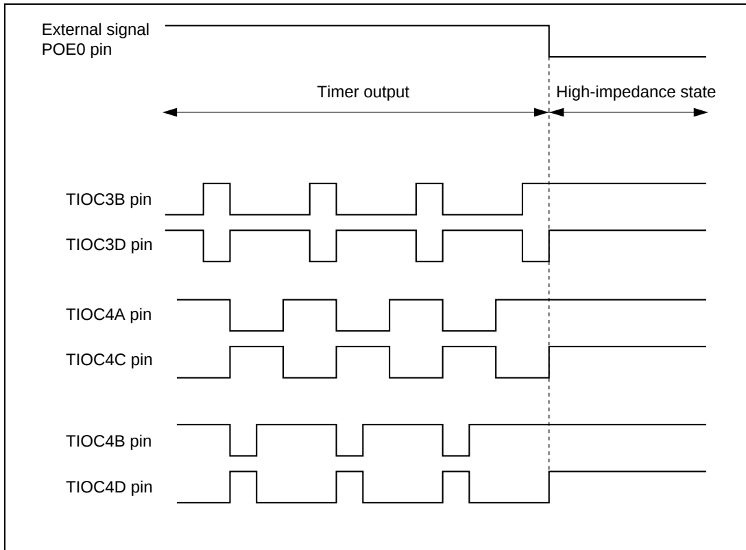
Figure 2-8-1 Example of Externally Triggered Timer Waveform Cutoff
