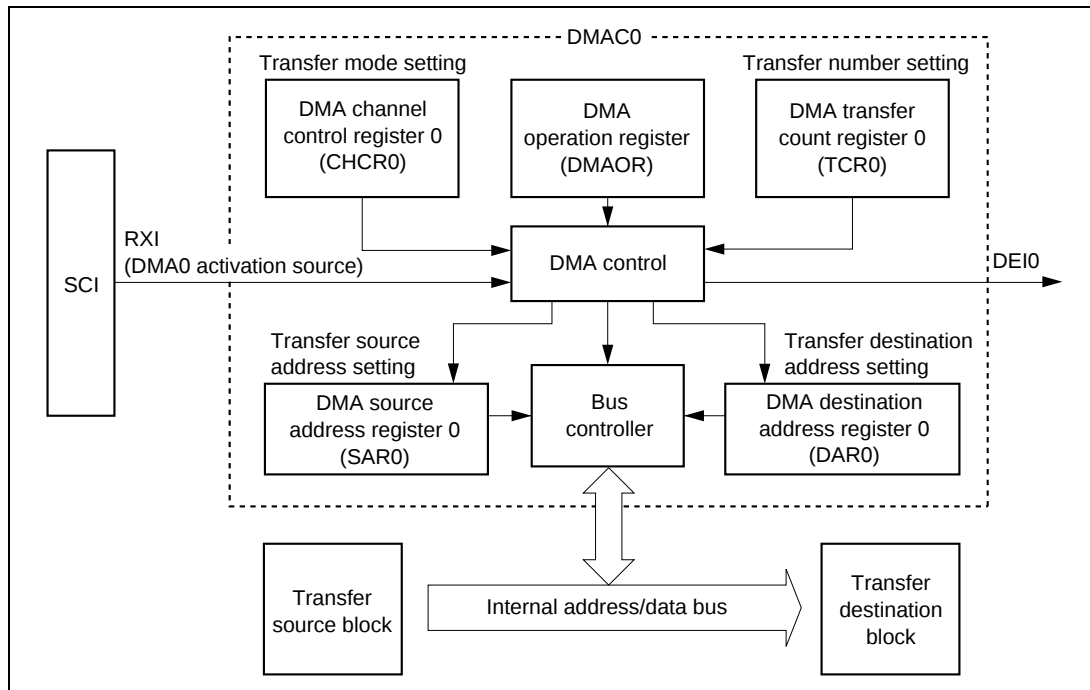
Figure 2-11-6 DMAC/ch0 Block Diagram
