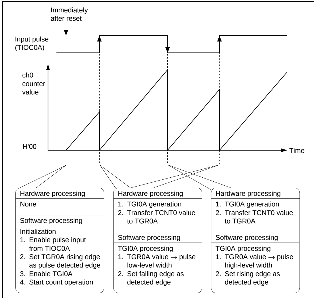
Figure 2-1-3 Principles of Pulse Width Measurement Operation
