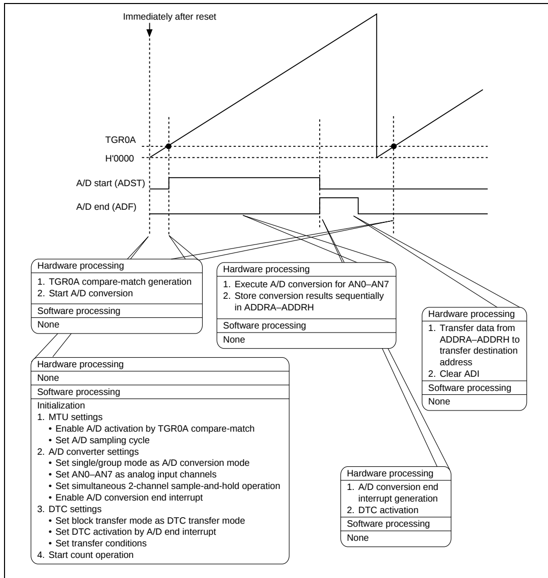
Figure 2-10-5 Principles of Pulse Width Measurement Operation
