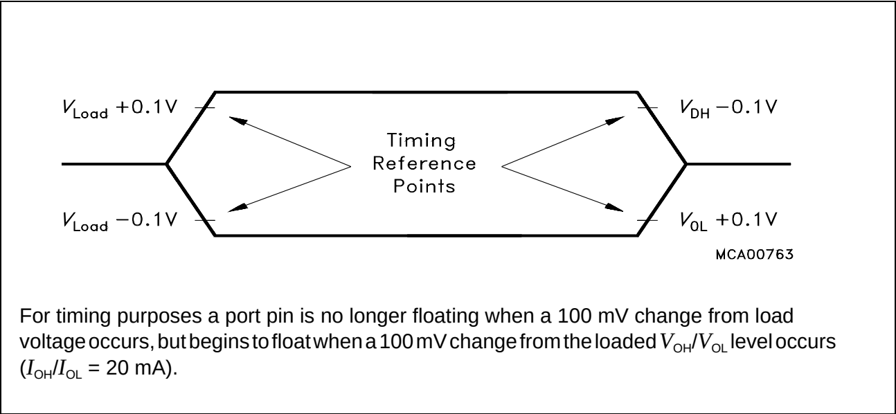
Figure 9 Float Waveforms
