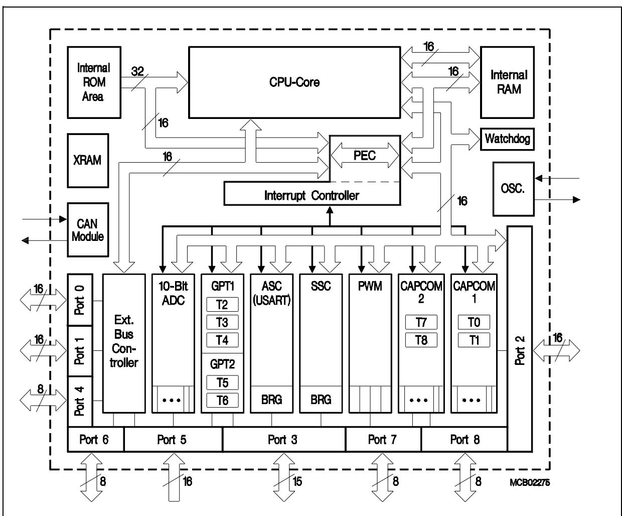
Figure 3 Block Diagram
