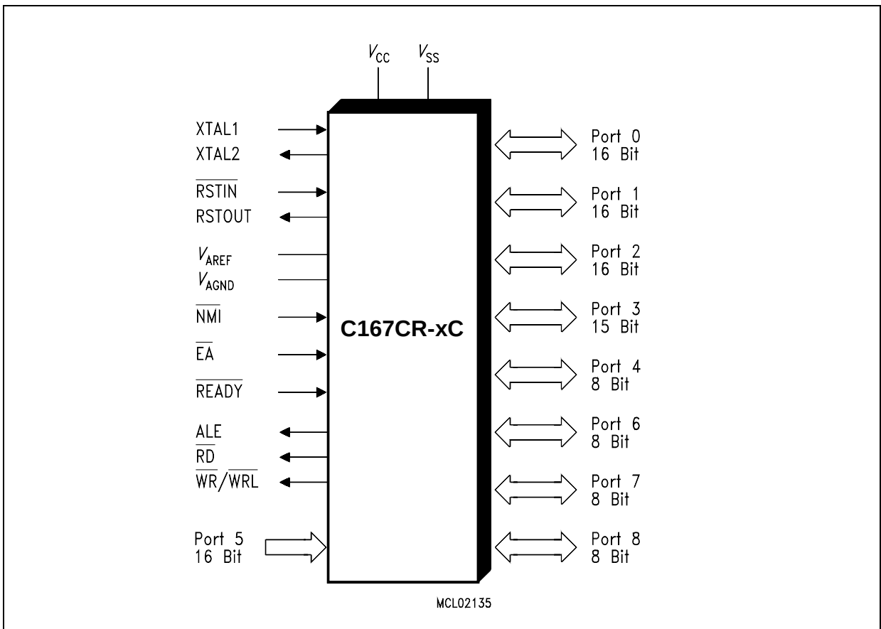
Figure 1 Logic Symbol
