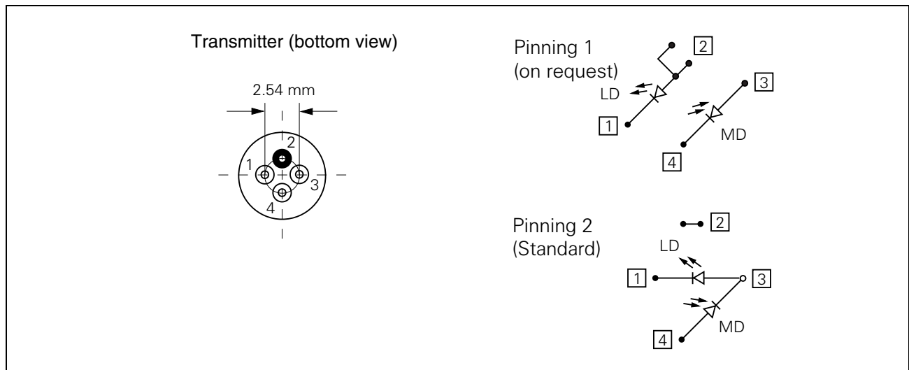
Figure 1 Transmitter
