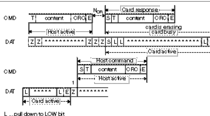
Timing of Erase Operation
