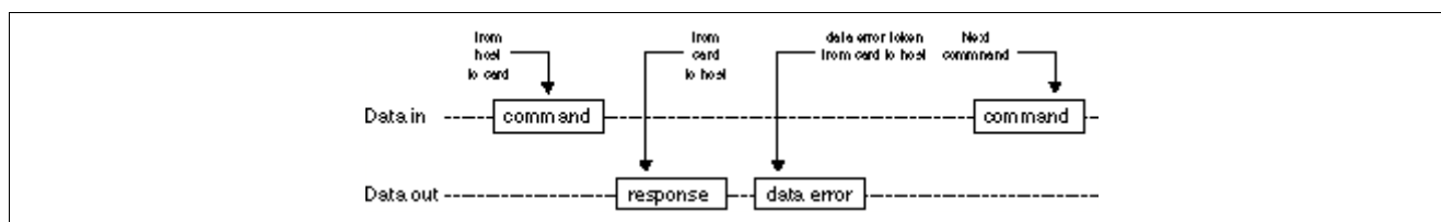
Read Operation-Data Error
