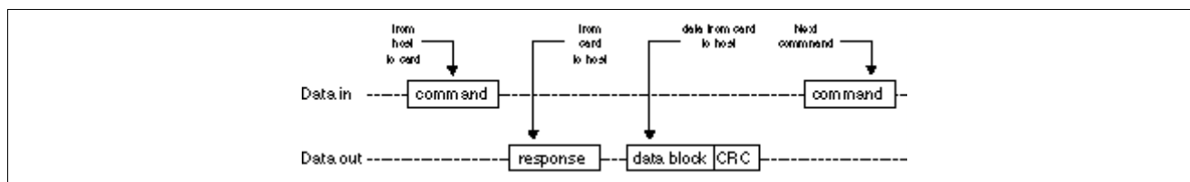
Read Operation
