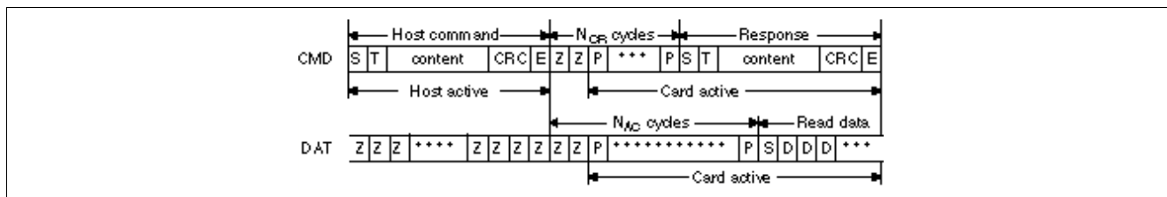
Data Read Timing (Data Transfer Mode)
