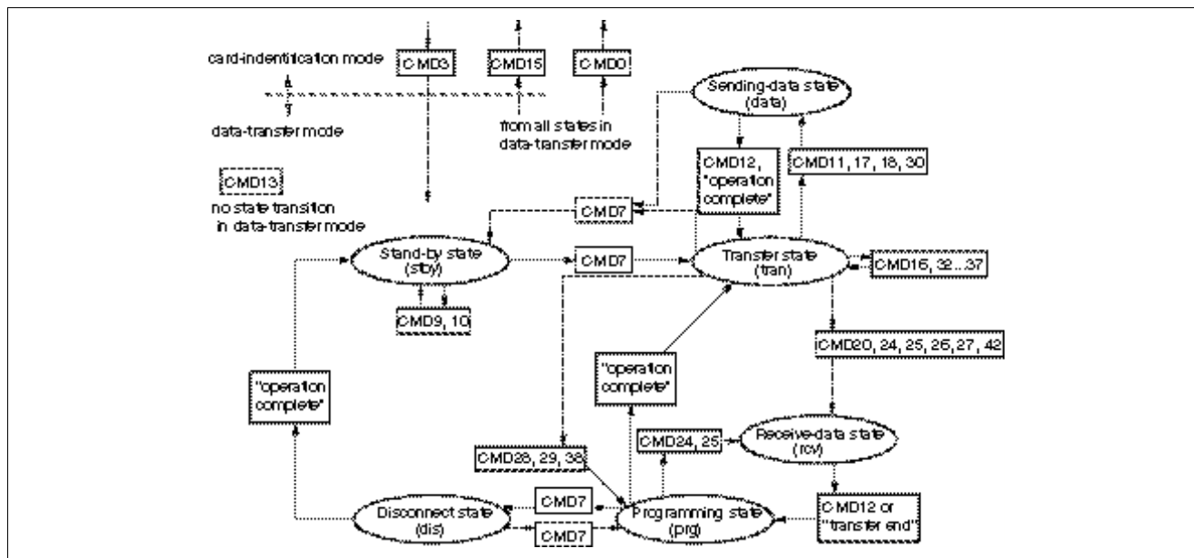
SLA F0064 H CA State Diagram (Data Transfer Mode)
