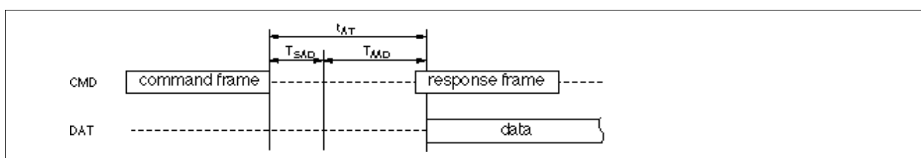
Access Time
