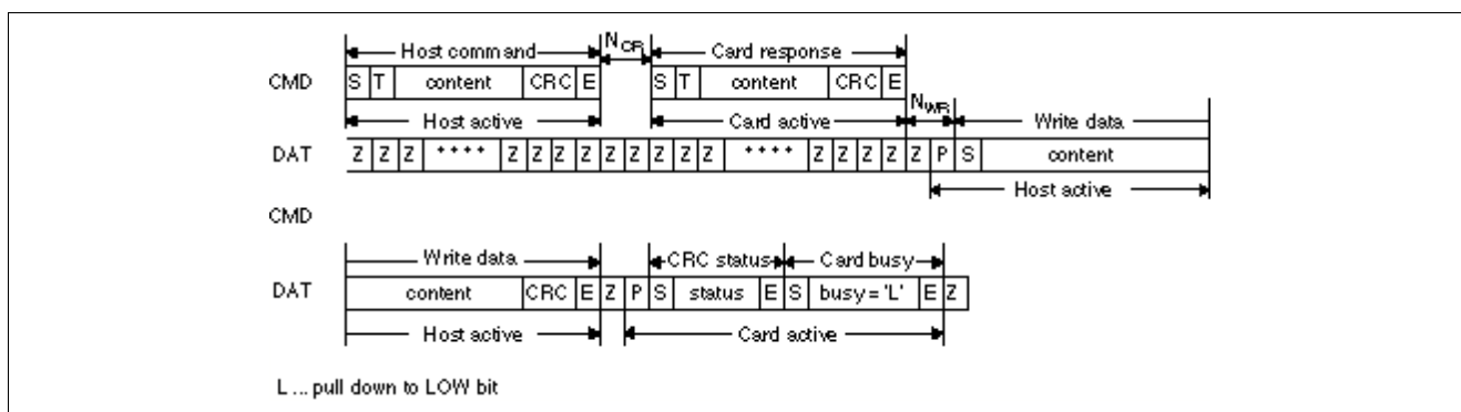
Timing of The Block Write Command
