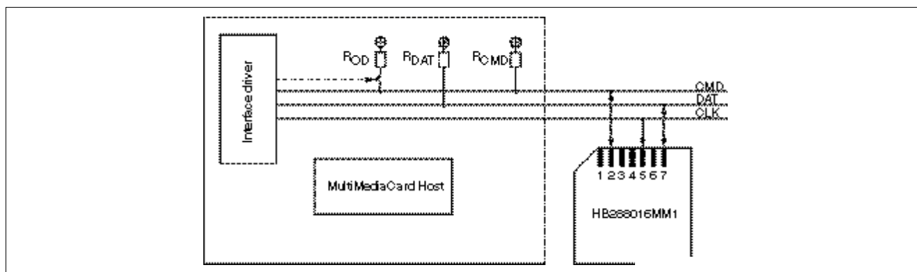
MultiMediaCard Mode Interface
