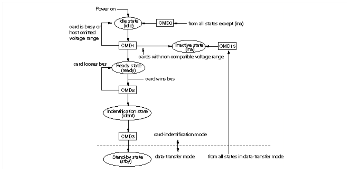
MultiMediaCard State Diagram (Card Identification Mode)
