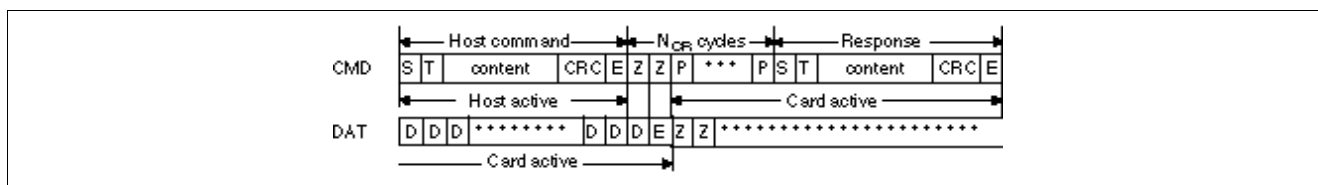
Timing of Stop Command (CMD12, Data Transfer Mode)
