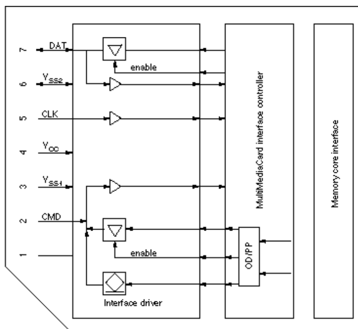
MultiMediaCard Mode I/O-drivers
