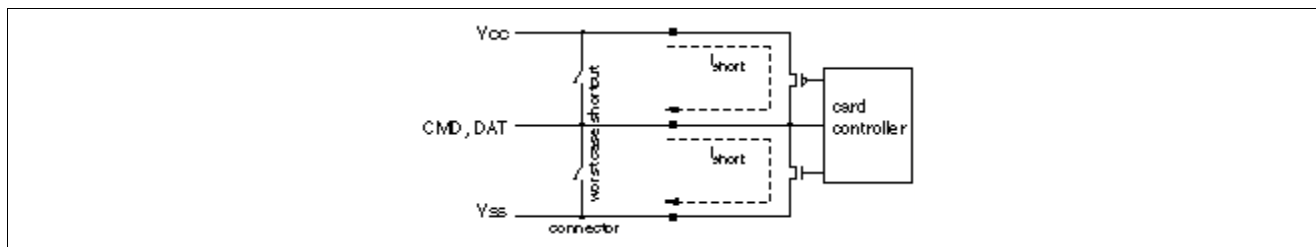
Short Cut Protection
