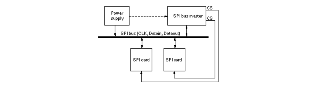
SPI Bus System
