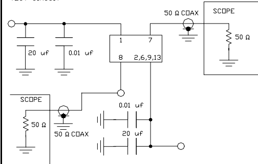
TEST CIRCUIT
