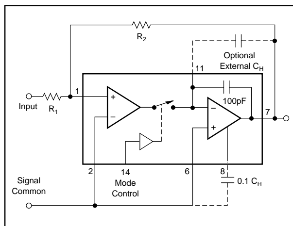
FIGURE 6. Inverting Configuration with Gain = -(R_2/R_1) .
