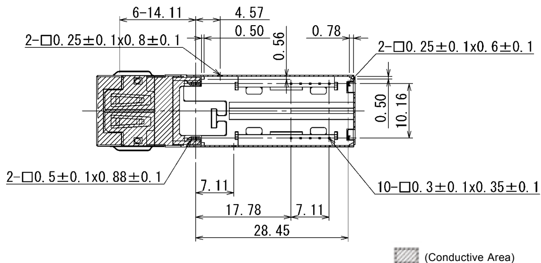
Figure 8. Bottom Side (SCM6428-GL-DN)
