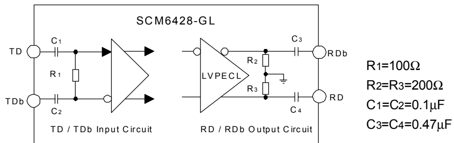
Figure 16. Data Input / Output Circuit
