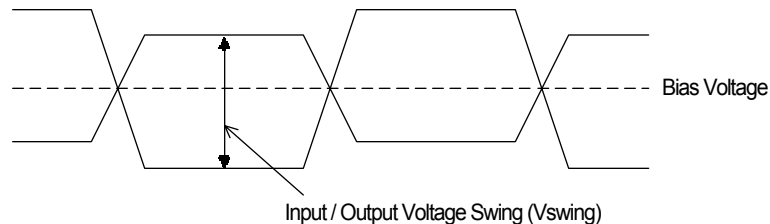
Figure 13. Definition of Differential Input / Output Voltage Swing
