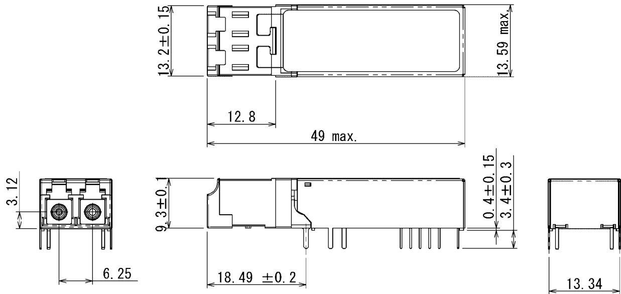
Figure 3. Outline Dimensions (SCM6428-GL-ZN)
