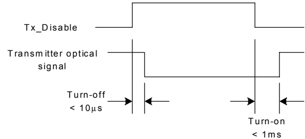
Figure 12. Definition of Turn-on / Turn-off Time
