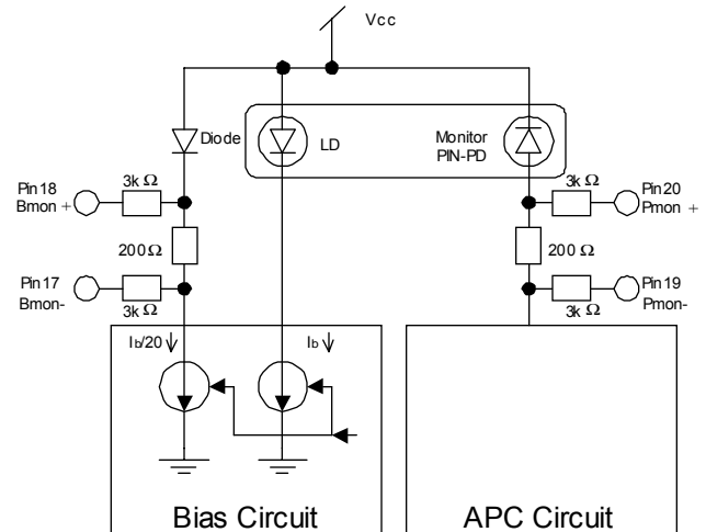
Figure 13. Bmon / Pmon Circuit Detail
