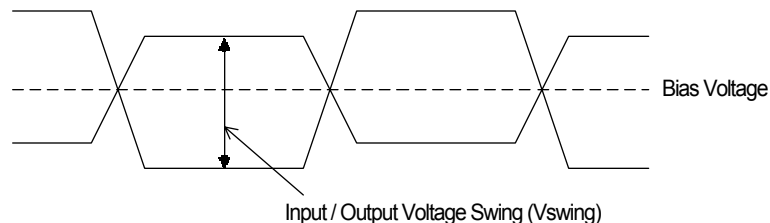
Figure 14. Definition of Differential Input / Output Voltage Swing
