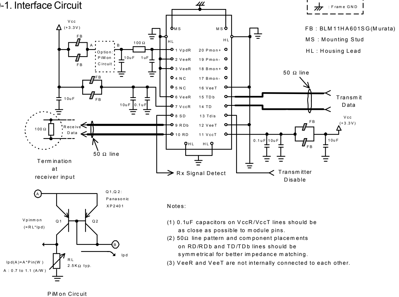
Figure 16. Recommended Interface Circuit
