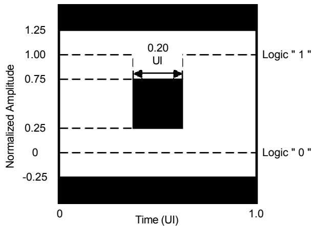
Figure 15. Optical Pulse Mask with Fourth Order Bessel-Thomson Filter Specified in ITU-T G.957
