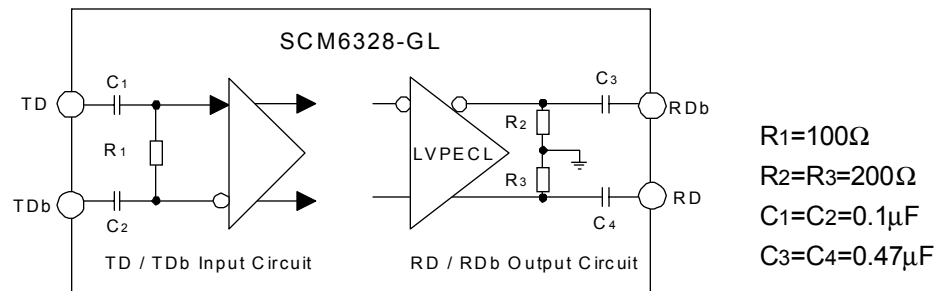
Figure 17. Data Input / Output Circuit
