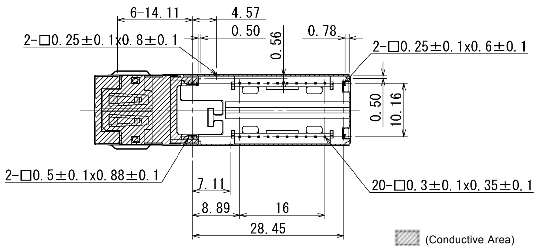
Figure 8. Bottom Side (SCM6328-GL-DN)
