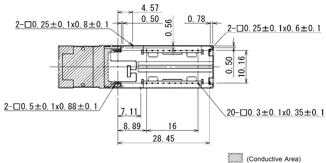
Figure 4. Bottom Side (SCM6328-GL-ZN)
