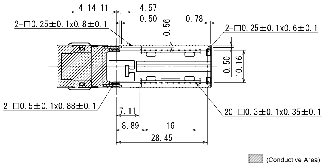
Figure 6. Bottom Side (SCM6328-GL-CN)
