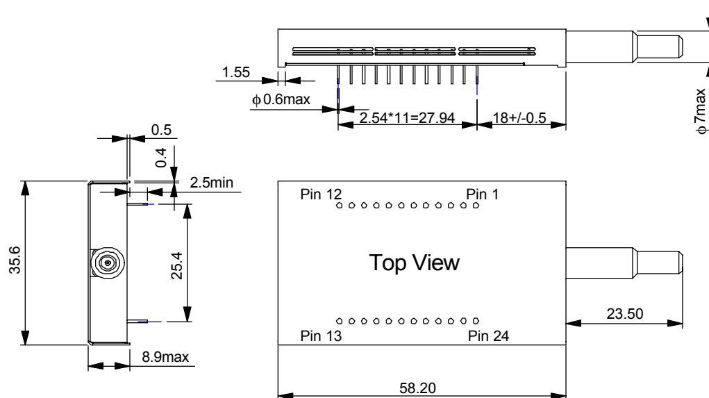
Figure 2 Package Dimension
