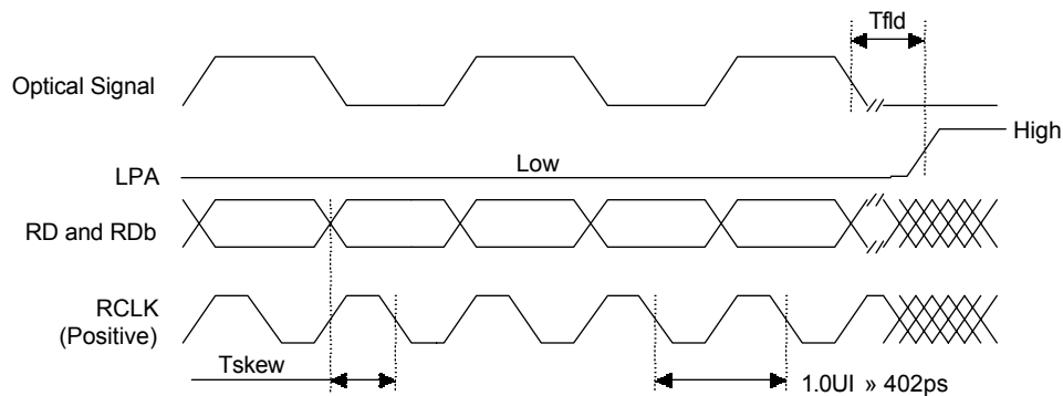
Figure 4 Output Timing Chart
