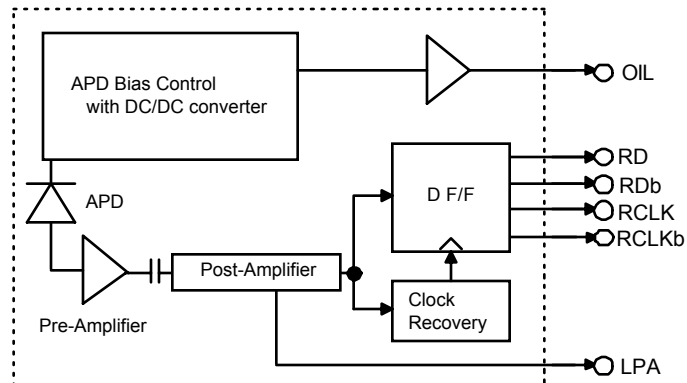
Figure 1 Block Diagram
