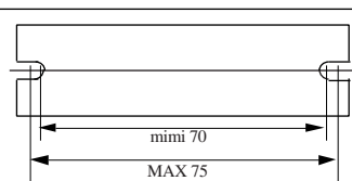
Plaque de Percage/Panel mounting
