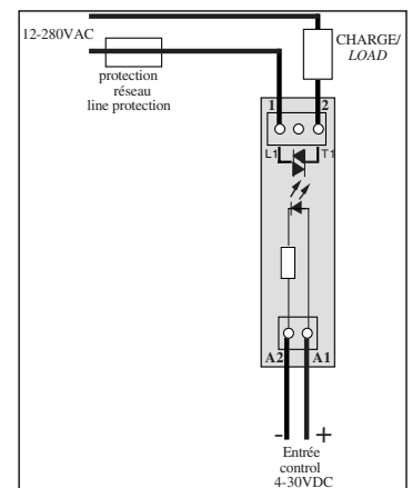
Application typique/Typical application
